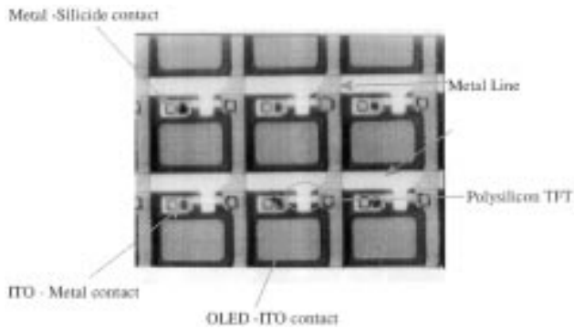
Fig. 9. Photograph of a completed 50\text{ }\mu\text{m} square single TFT pixel (top view).
