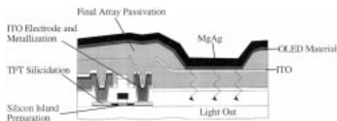
Fig. 2. AM-OLED array process overview.
