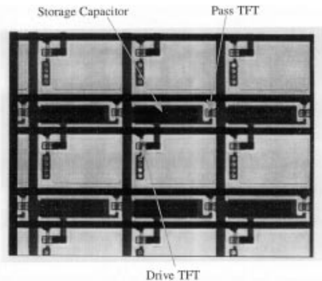
Fig. 10. Photograph of completed 100\text{ }\mu\text{m} square pixel having the 2-TFT design. The pass TFT, storage capacitor, and drive TFT are indicated.
