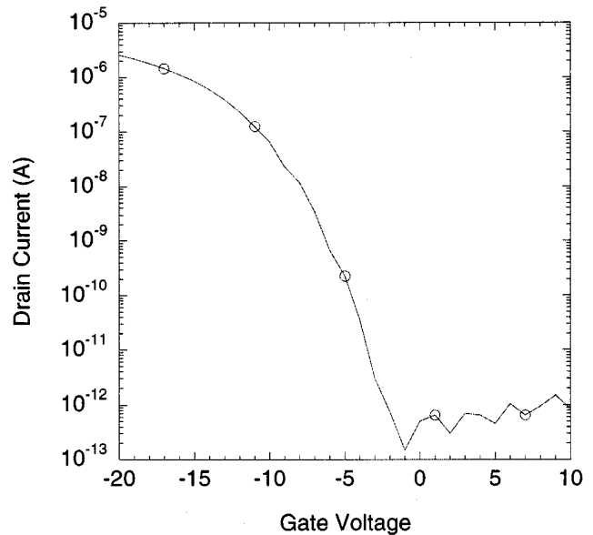
Fig. 11. P-channel pixel TFT transfer characteristics. W/L = 4\text{ }\mu\text{m}/8\text{ }\mu\text{m} , V_{DS} = -1\text{ V} .
