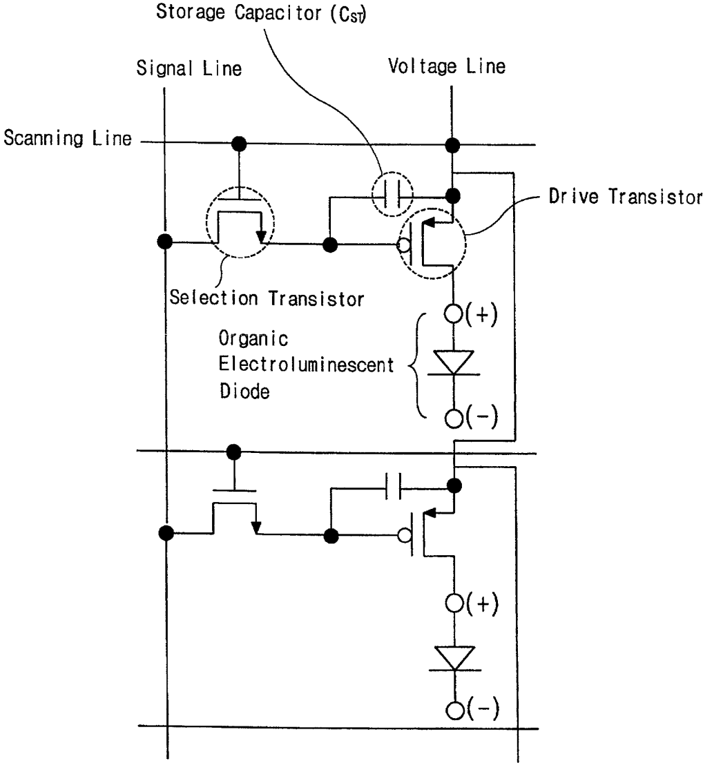
FIG. 1 (RELATED ART)
