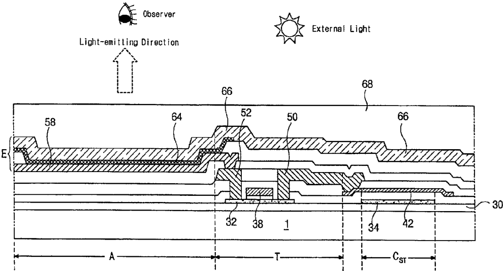
FIG. 2 (RELATED ART)
