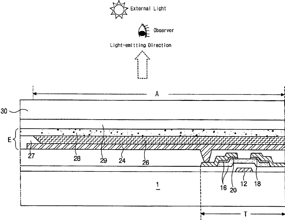
FIG. 3 (RELATED ART)
