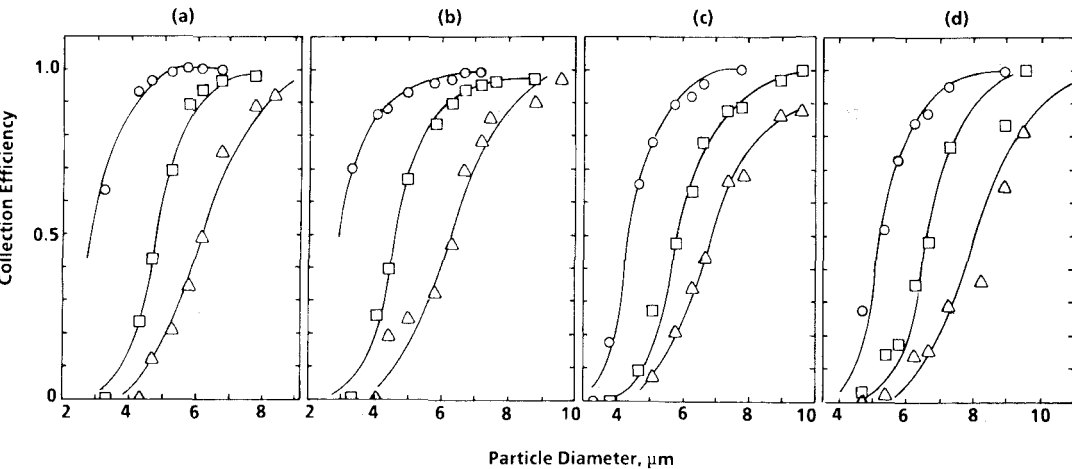
FIGURE 4. Measured collection efficiency as a function of particle size for (a) cyclone II-1, (b) cyclone II-2, (c) cyclone II-3, and (d) cyclone II-4. (○) 18.4 L/min; (□) 12.4 L/min; (△) 8.8 L/min.
