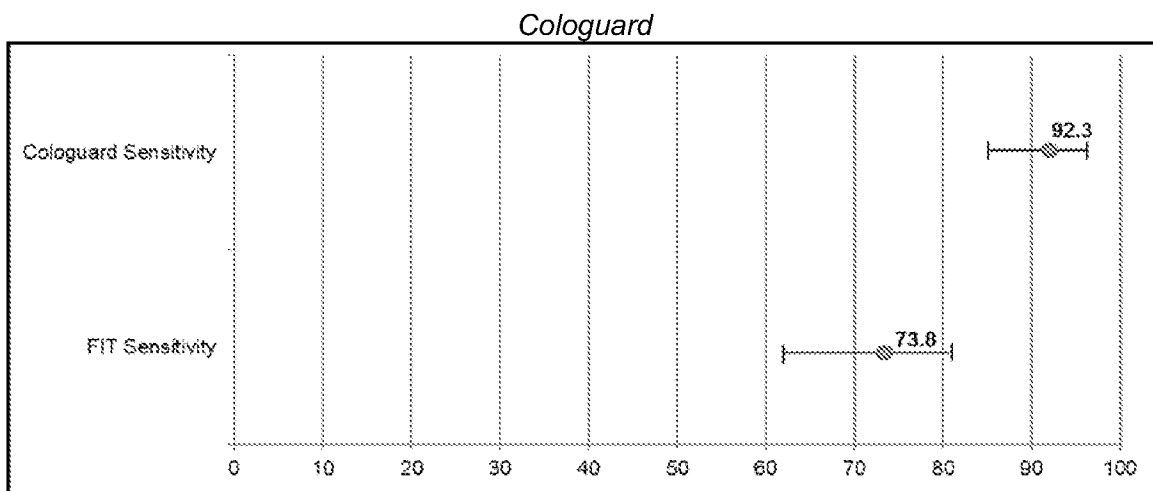
Figure 1: CRC Sensitivity
