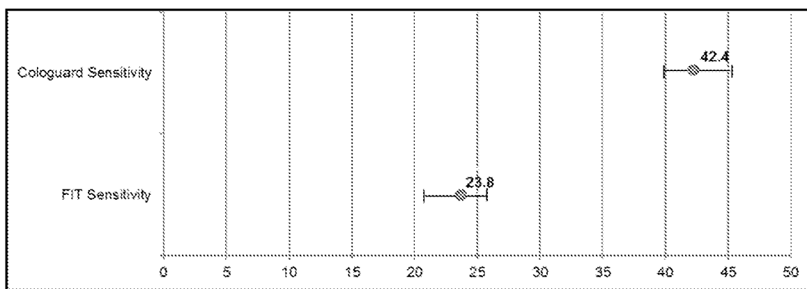
Figure 2: AA Sensitivity
