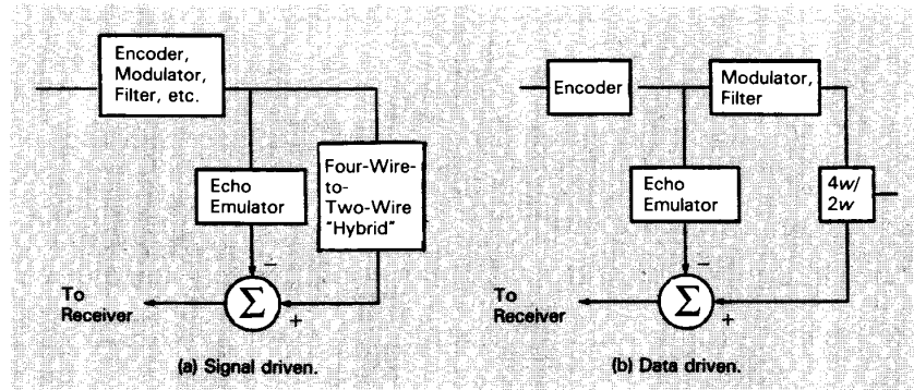
Fig. 8. Echo cancelers.
