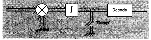
Fig. 4. Integrate and dump detection for QASK.
