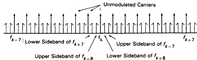
Fig. 5. Multicarrier spectrum with sidebands resulting from 60 Hz phase jitter.
