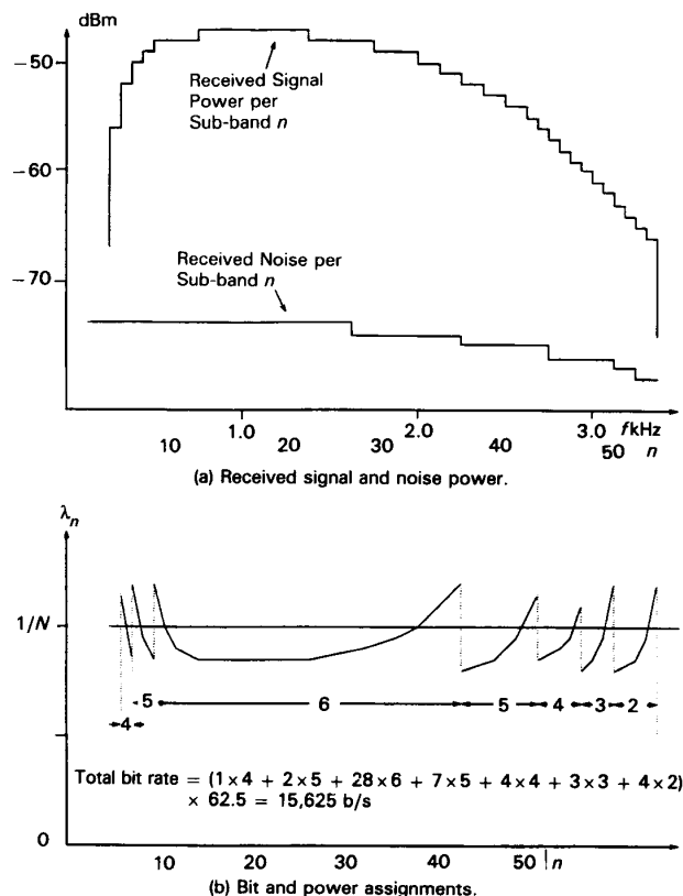
Fig. 3. Adaptive loading for a badly distorted GSTN channel.
