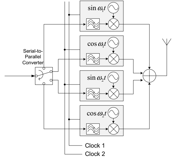
Figure 3: The OFDM scheme, proposed by Chang, implements Fourier transforms to bestow orthogonality amongst the subcarriers. The evolution from the FDM parallel transmission to the first OFDM scheme can be seen by replacing the narrowband transmitters, employed by an FDM scheme, with an analog implementation of Fourier transforms.
