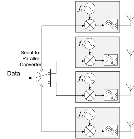
Figure 2: A parallel transmission scheme utilizing FDM is implemented by the use of a serial-to-parallel converter and multiple narrowband transmitters.
