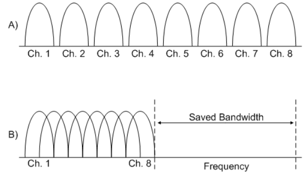
Figure 1: A) The frequency spectrum of eight channels shown utilizing frequency division multiplexing. Parallel transmitters are employed in which guard bands are placed between sub-carriers. B) The frequency spectrum of OFDM is shown where sub-channels are orthogonal to the adjacent channels. The percentage of bandwidth used to transmit the same data is reduced by 50%.
