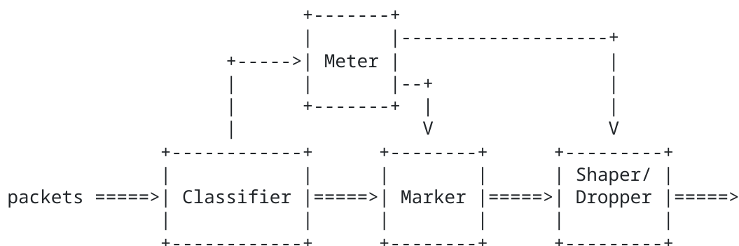
Fig. 1: Logical View of a Packet Classifier and Traffic Conditioner
