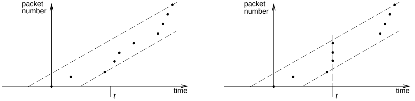
Figure 3: An example of perturbation. Left: A sequence \sigma . Right: \sigma(5:t) . Note that in \sigma(5:t) packets 3, 4, 5 were moved with respect to \sigma .
