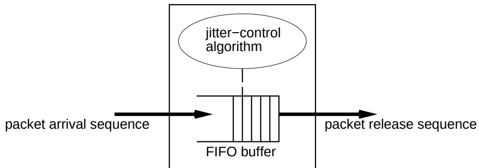
Figure 1: Abstract node model. The jitter control algorithm controls packet release from the buffer, based on the arrival sequence.
