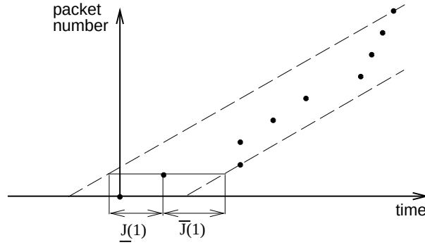
Figure 2: An example for oriented jitter bounds. A point at coordinates (x, y) denotes that packet y is released at time x . The slope of the dashed lines is 1/X_a .
