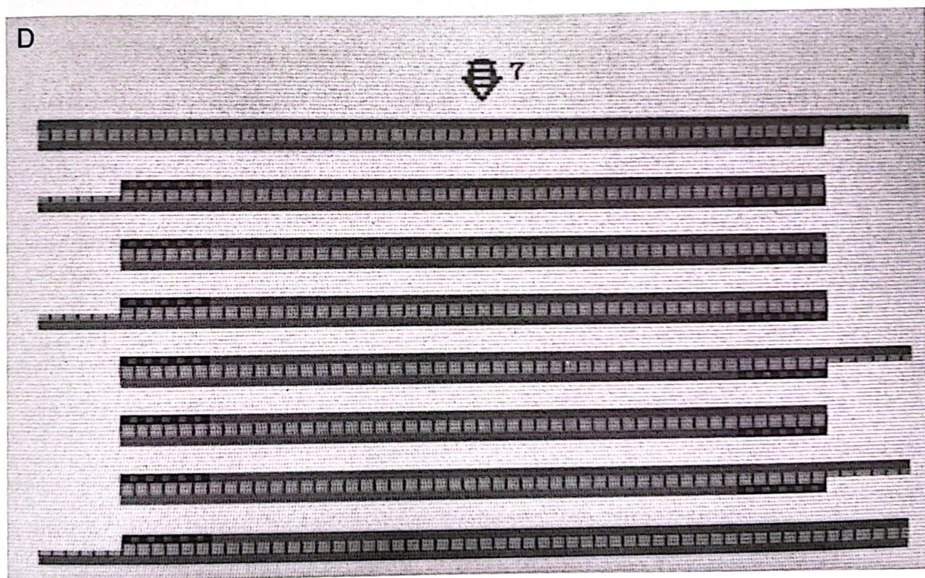
Figure 1. Three complete cycles of the polymerase chain reaction resulting in the eightfold amplification of a template sequence defined by the 5' ends of two primers hybridized to different strands of the template are depicted above. The first cycle is shown in detail as reactions 1, 2, and 3. The second cycle is depicted in less detail as reactions 4 and 5, and the third cycle, as reactions 6 and 7. By cycle 3, a double-stranded DNA fragment is produced that has discrete termini, and thus the targeted sequence has been extracted from its source as well as amplified.
