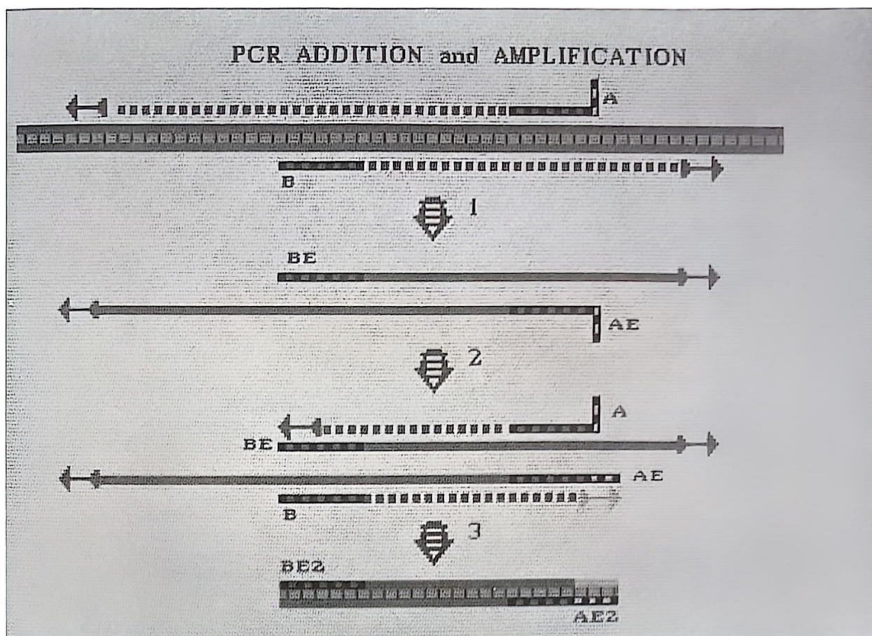
Figure 3. Addition of the nonhomologous sequence on the 5' end of oligonucleotide A results, after the first PCR cycle, in the incorporation of this nonhomologous sequence into extension product AE, which, in a later cycle as template for B, directs the synthesis of BE2 that together with AE2 comprises the double-stranded DNA fragment AE2:BE2. This fragment will accumulate exponentially with further cycles.
