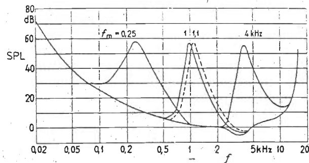
Fig. 3. Masking thresholds of narrow-band noise signals centred at various frequencies f_m .
