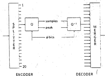
Fig. 4. Subband coding system with 20 subbands.
