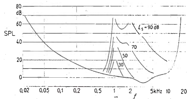
Fig. 2. Masking thresholds of pure tones of 1.0 kHz at various SPLs L_s .
