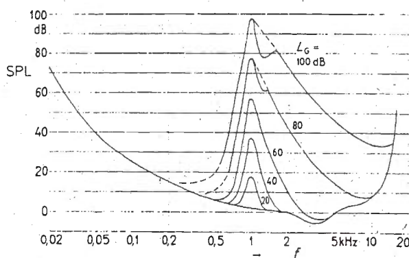
Fig. 1. Hearing threshold (lower curve) and masking thresholds of narrow-band noise signals centred at 1.0 kHz at various SPLs L_G .
