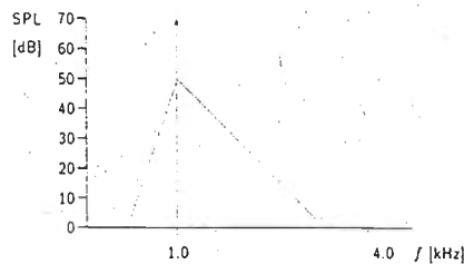
Fig. 5. Masking threshold as a function of frequency.
