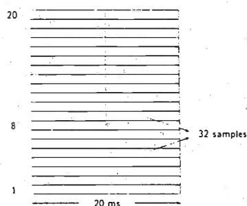
Fig. 8. Allocation window for a 20-band system.
