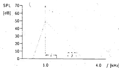
Fig. 7. Masking of subbands at higher frequencies.
