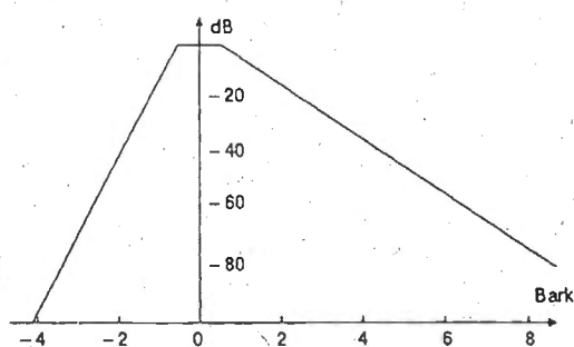
Figure 2 Basilar membrane spreading function
