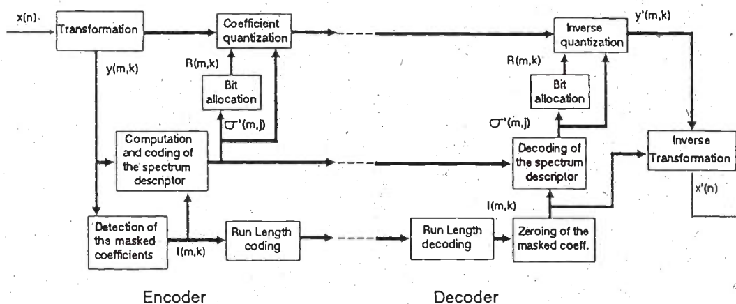
Figure 1 General Scheme of the Algorithm
