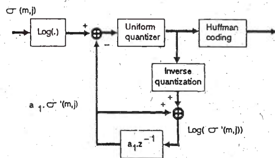
Figure 3 Predictive coding of the spectrum descriptor
