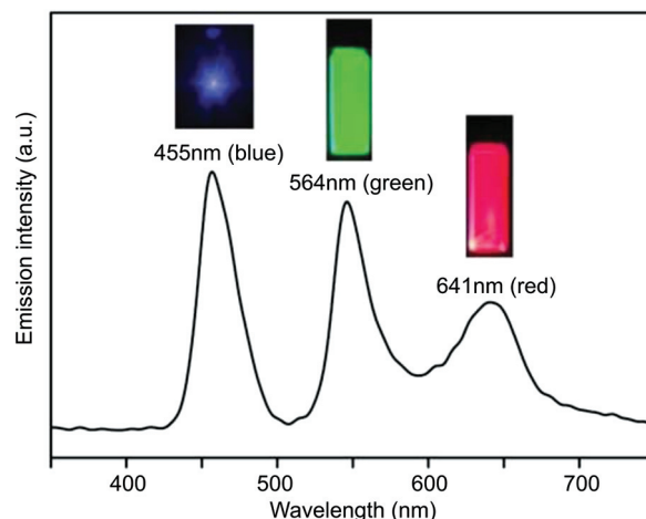
Figure 18. (Color online) Three-band white LED combining a blue InGaN chip, green-emitting CdSe-ZnSe QDs and red-emitting CdSe-ZnSe QDs. Adapted from Ref. 160, (© 2006 IEEE) Reproduced with permission.
