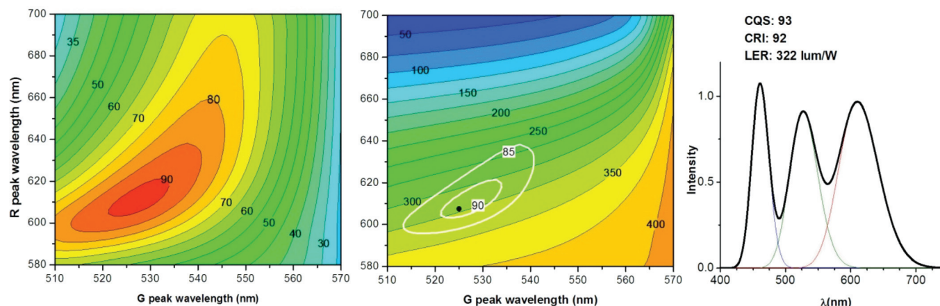
Figure 7. (Color online) CQS (left) and LER (center) for a white light source with CCT of 4500 K consisting of two variable emission bands (FWHM of 50 nm (G) and 70 nm (R)) and one emission band fixed at 460 nm (FWHM of 30 nm). On the center image, the contour lines for CQS equal to 85 and 90 are superposed in white. Right: The emission spectrum indicated by the black dot in the center image.
