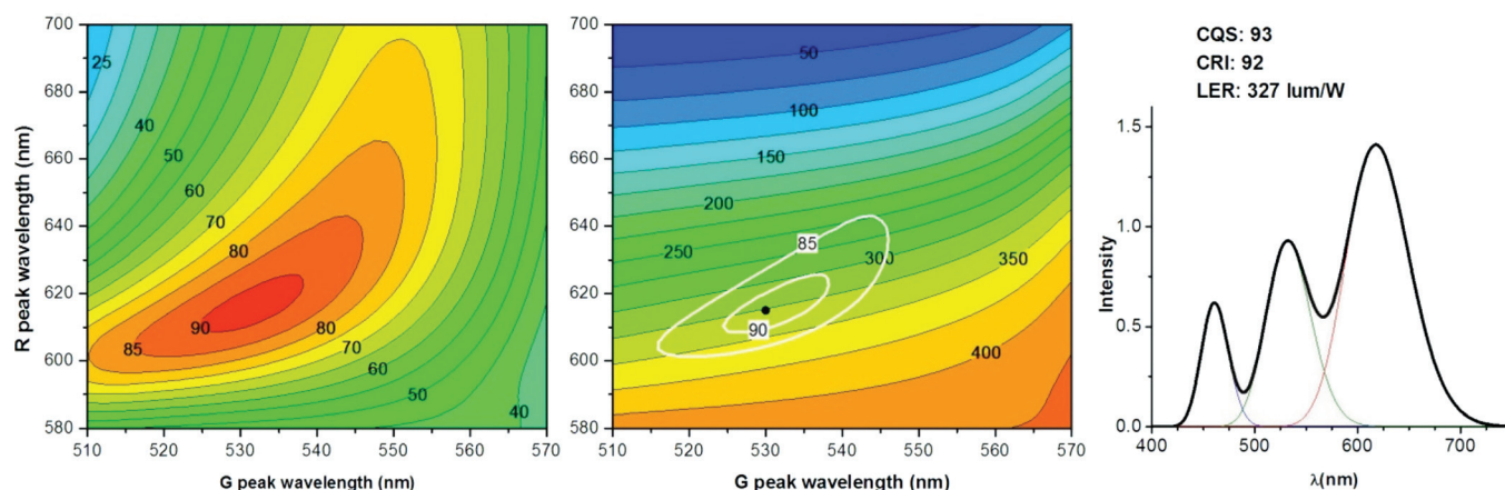
Figure 6. (Color online) CQS (left) and LER (center) for a white light source with CCT of 3000 K consisting of two variable emission bands (FWHM of 50 nm (G) and 70 nm (R)) and one emission band fixed at 460 nm (FWHM of 30 nm). On the center image, the contour lines for CQS equal to 85 and 90 are superposed in white. Right: The emission spectrum indicated by the black dot in the center image.
