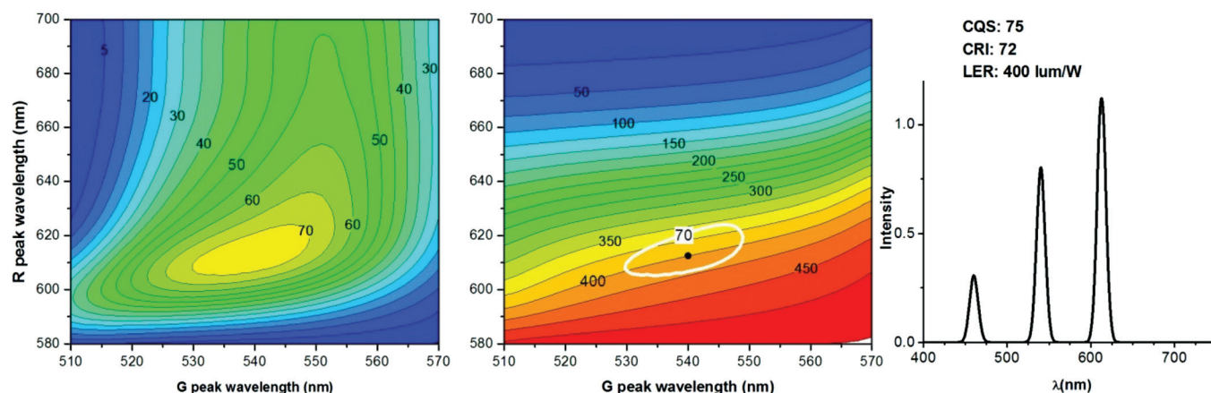
Figure 4. (Color online) CQS (left) and LER (center) for a white light source with CCT of 3000 K consisting of two variable emission bands (FWHM of 10 nm) and one emission band fixed at 460 nm (FWHM of 10 nm). On the center image, the contour line for CQS equal to 70 is superposed in white. Right: The emission spectrum indicated by the black dot in the center image.
