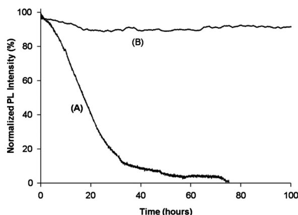
Figure 9. Accelerated aging at 80% relative humidity and 80°C of (A) uncoated \text{CaS:Eu}^{2+} particles and (B) coated with sol-gel prepared \text{Al}_2\text{O}_3 . Photoluminescence intensity was measured in situ upon excitation with a 440 nm LED. 60 Copyright (2010), with permission from Elsevier.
