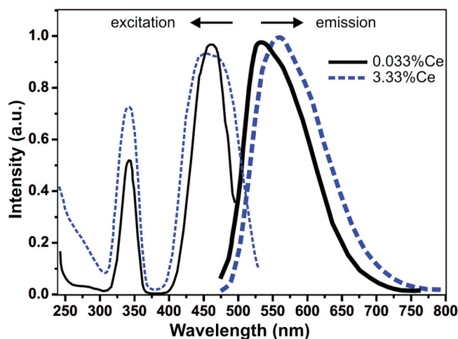
Figure 13. (Color online) Emission and excitation spectra for \text{Y}_3\text{Al}_5\text{O}_{12}:\text{Ce}[0.033\%] and \text{Y}_3\text{Al}_5\text{O}_{12}:\text{Ce}[3.3\%] . Adapted from Ref. 45, copyright 2009 American Chemical Society.
