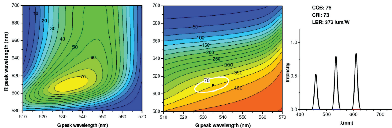
Figure 5. (Color online) CQS (left) and LER (center) for a white light source with CCT of 4500 K consisting of two variable emission bands (FWHM of 10 nm) and one emission band fixed at 460 nm (FWHM of 10 nm). On the center image, the contour line for CQS equal to 70 is superposed in white. Right: The emission spectrum indicated by the black dot in the center image.
