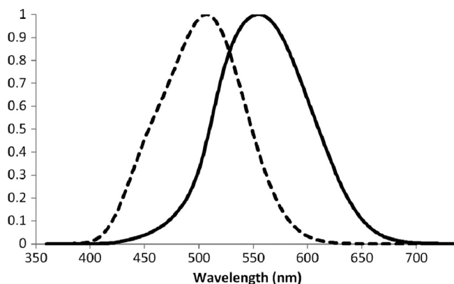
Figure 2. Normalized spectral eye sensitivity curves for photopic vision V(\lambda) (full line) and scotopic vision V'(\lambda) (dashed line), as specified by the CIE.
