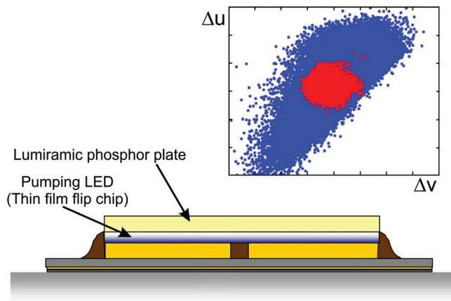
Figure 16. (Color online) (Bottom) Schematic view of a white LED with a Lumiramic (YAG:Ce) phosphor plate on top of the pumping LED. (Top) Color deviation for LUXEON LEDs (Philips) from the intended device color for >150 K phosphor-based LEDs (blue) and when using ceramic phosphor plates (red). Adapted from Ref. 143, reproduced with permission.
