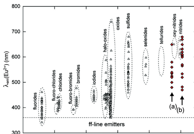
Figure 15. (Color online) Emission wavelength of \text{Eu}^{2+} -doped compounds, adapted from Ref. 88. Data (in red) are shown for recently reported \text{Eu}^{2+} -doped (a) oxynitride and (b) nitride phosphors. Copyright (2003), with permission from Elsevier.
