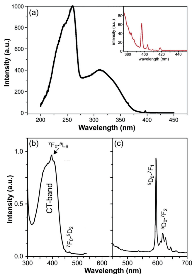
Figure 14. (Color online) (a) Excitation spectrum for the red \text{Eu}^{3+} emission in \text{Y}_2\text{O}_3\text{S} . Adapted from Ref. 103, copyright (2008), with permission from Elsevier. (b) Excitation ( \lambda_{\text{em}} = 594 nm) and (c) emission ( \lambda_{\text{exc}} = 395 nm) spectra for orange-emitting \text{Ba}_{1.9}\text{Eu}_{0.05}\text{Li}_{0.05}\text{CaMoO}_6 . Adapted from Ref. 104, reproduced by permission of The Electrochemical Society.
