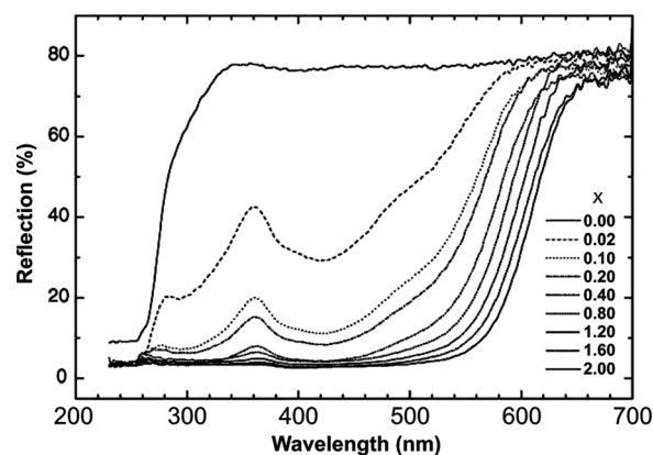
Figure 12. Diffuse reflection spectra for \text{Sr}_{2-x}\text{Eu}_x\text{Si}_5\text{N}_8 . Adapted from Ref. 77, copyright (2006), with permission from Elsevier.
