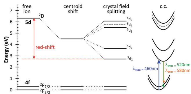
Figure 11. (Color online) Energy level diagram for the free (gaseous) \text{Ce}^{3+} ion and for \text{Y}_3\text{Al}_5\text{O}_{12}:\text{Ce}^{3+} , where the effects of the centroid shift and the crystal field on the degenerate 5d level are indicated. For the ^2\text{D} levels of the free ion, the average energy is indicated. The position of the ^5\text{d}_4 level is uncertain. 87 On the right a simplified configurational coordinate diagram (c.c.) is shown.
