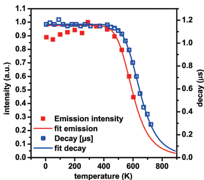
Figure 8. (Color online) Temperature dependence of the integrated emission intensity and luminescence decay times for \text{SrSi}_2\text{O}_2\text{N}_2:\text{Eu}^{2+}[2\%] . Adapted from Ref. 50, Copyright 2009 American Chemical.
