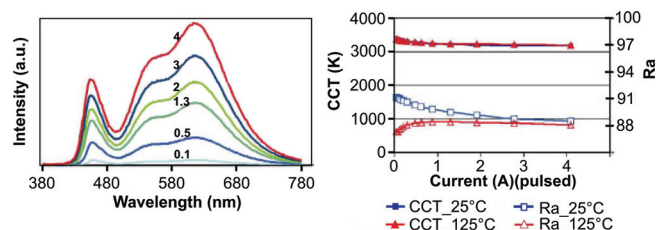
Figure 17. (Color online) (left) Dependency on drive current of a 2-pc-LED emission, using two (oxy)nitride phosphors, up to 4A (2 W/mm 2 optical pump power) and (right) CCT and Ra with drive current and temperature (shown for 25 and 125°C). Adapted from Ref. 40, Copyright Wiley-VCH Verlag GmbH & Co. KGaA. Reproduced with permission.
