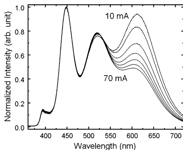
Figure 10. Normalized emission spectra for a white LED as function of the driving current. The white LED is composed of a UV pumping LED, blue and green \text{Eu}^{2+} phosphors and red \text{Eu}^{2+}\text{-Mn}^{2+} phosphor. Adapted from Ref. 64, reproduced by permission of The Electrochemical Society.
