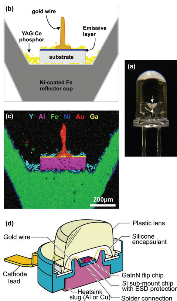
Figure 3. (Color online) (a) 5 mm, 20 mA white LED, (b) schematic structure of the LED's cross-section along the plane perpendicular to the image (a) and indicated by the white arrows, (c) elemental mapping of selected elements using EDX (energy-dispersive x-ray analysis), with the maps for Y, Al and Ga indicating the \text{Y}_3\text{Al}_5\text{O}_{12}:\text{Ce} phosphor powder, the sapphire substrate and the (Ga,In)N diode, respectively. Adapted from Ref. 131. (d) Schematic structure of a high-power package. Note the improved thermal management and the presence of an electrostatic discharge (ESD) protection. Adapted from Ref. 132, reproduced with permission.
