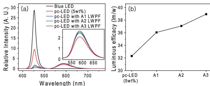
Fig. 4. (a) The equal-power spectra of a conventional blue-pumped pc-LED and pc-LEDs with three types of LWPFs (phosphor concentration: 5 wt%). The enlarged view shows the spectra at the amber region. The black line shows the spectra of only the conventional blue LED. (b) The luminous efficacy of pc-LEDs (5 wt%) of a conventional blue-pumped pc-LED and pc-LEDs with three types of LWPFs.
