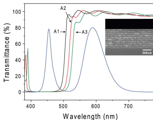
Fig. 3. Measured transmittance spectra of the three different LWPFs [0.5H(L)0.5H]^9 (L: low index layer, \text{SiO}_2 , H: high index layer, \text{TiO}_2 ) on glass substrates, and the normalized electroluminescent (EL) spectrum of pc-LED with silicate amber powder phosphor (phosphor concentration 20 wt%). The inset shows a side-view scanning electron microscopy (SEM) image of the nine periods of the [0.5H(L)0.5H] films coated onto a glass substrate.
