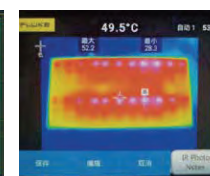
Surface Temperature
