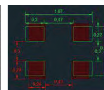
Pad matching
