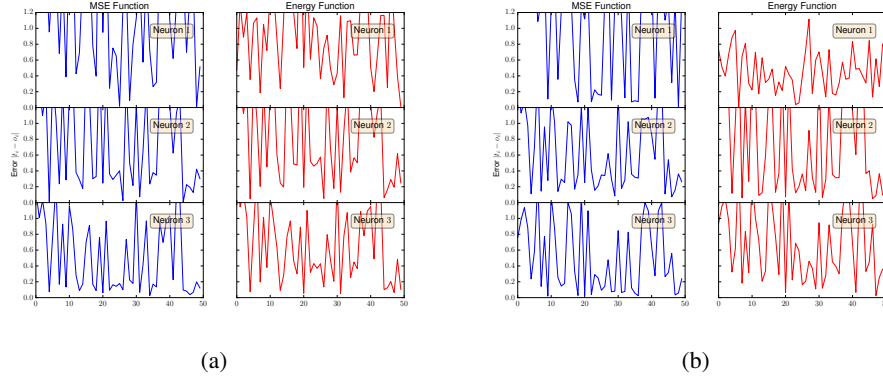
Figure 5: Errors of each output neuron |t_i - o_i| for a random order of test pairs.
