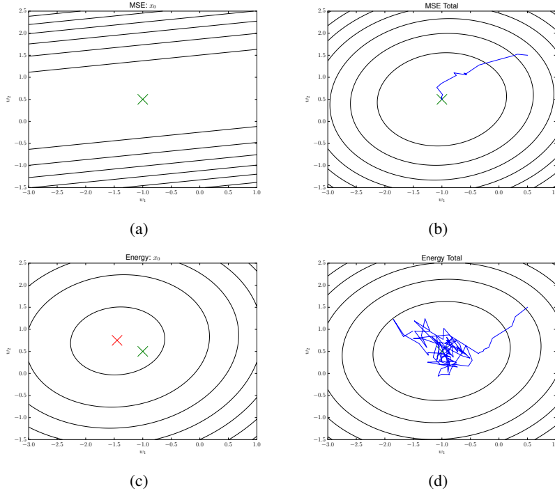
Figure 1: The error surfaces in weight space for a single linear neuron with two inputs. The observations \{\mathbf{x}, t\} have a single solution in weight space with zero MSE. (a) A single observation \mathbf{x}_0, t_0 for the MSE function, corresponding to a trench. The green ‘X’ denotes the minimum of the total MSE function. (b) The total MSE function for all data sets. A sample stochastic gradient descent path from a random starting point is shown. (c) As (a), for the energy function. The red ‘X’ denotes the minimum of this observations energy function. (d) As (b), for the energy function.
