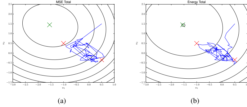
Figure 2: Total error surfaces for a set of observations \{\mathbf{x}, t\} that consists of two subsets, each with a single solution in weight space with zero MSE. The green ‘X’ denotes the minimum of the total error function. The red ‘X’ denote the exact solutions of the two subsets. (a) The total MSE function for all data sets. A sample stochastic gradient descent path from a random starting point is shown. (b) As (a), for the energy function.
