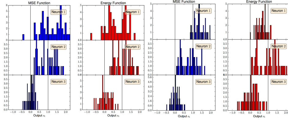
Figure 4: Histograms of the three output neurons for test pairs. Shown for networks with one hidden layer (left two panels) and three hidden layers (right two panels).
