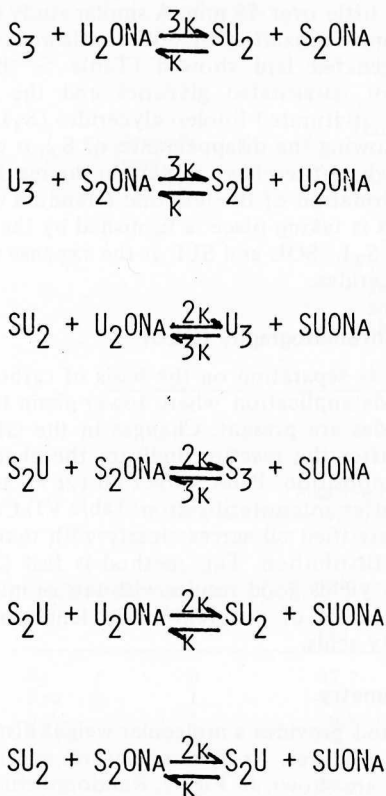
FIG. 6. Chain reaction initiated by diglycerinate for fatty acid interchange.
