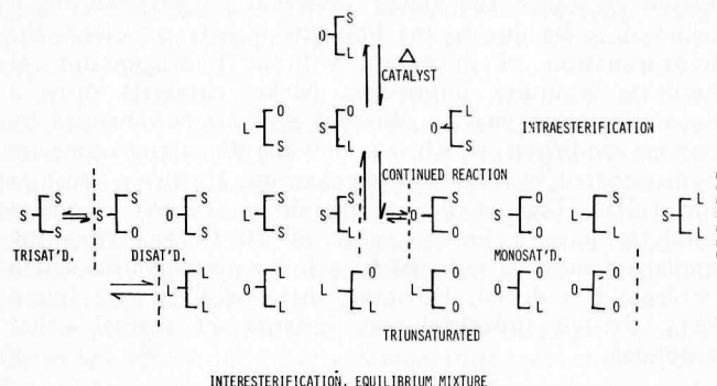
FIG. 1. Formation of glycerides during molecular rearrangement.
