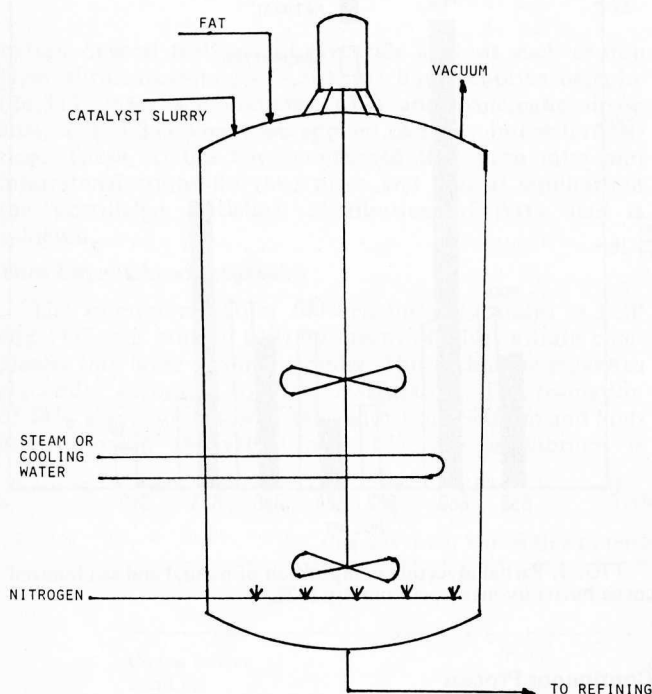
FIG. 10. Batch reactor for interesterification.
