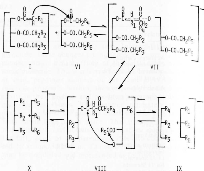
FIG. 4. Mechanism for intramolecular ester-ester interchange.
