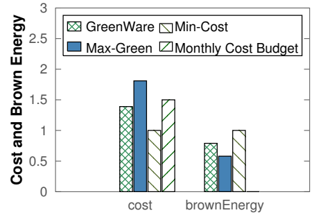
Fig. 8. Comparison between GreenWare and baselines with respect to Nov. 2007 Wikipeida trace
