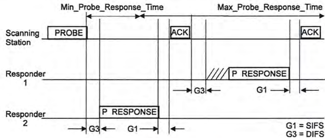
Figure 10-3—Probe response
