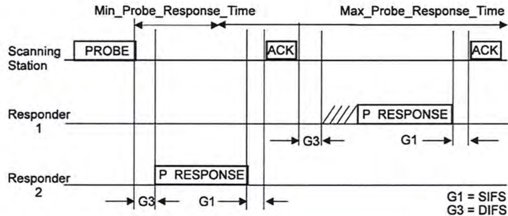
Figure 10-3—Probe response
