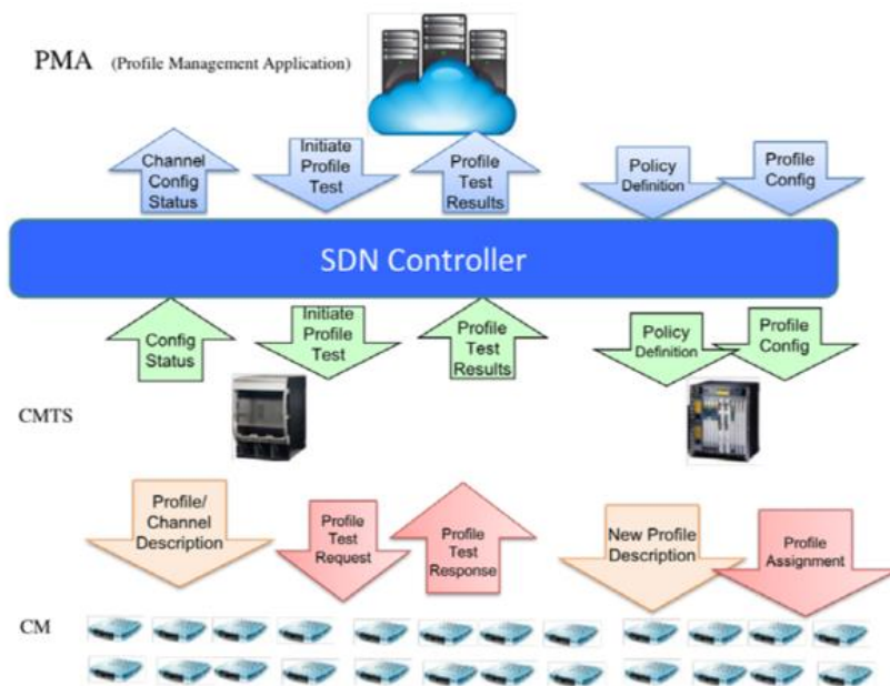
Figure 2 - PMA Architecture w SDN Controller
