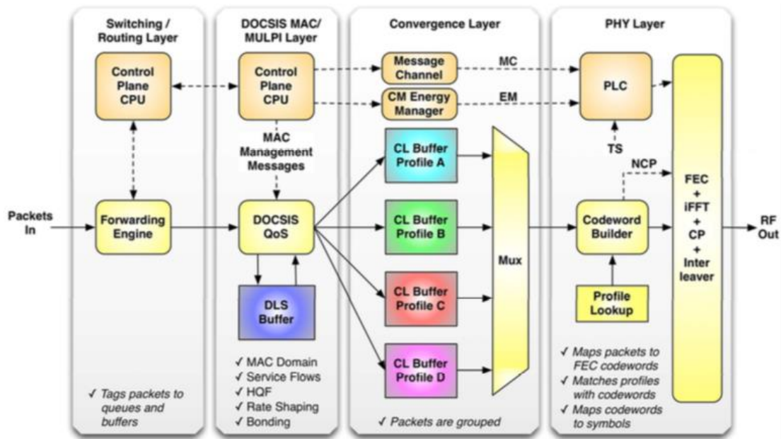
Figure 89 - Downstream Convergence Layer Block Diagram
