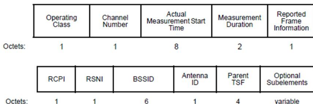
Figure 9-199—Measurement Report field format for Beacon report
