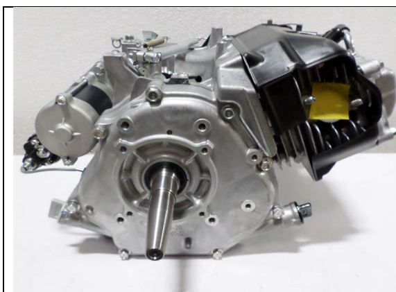
Tapered engine shafts
