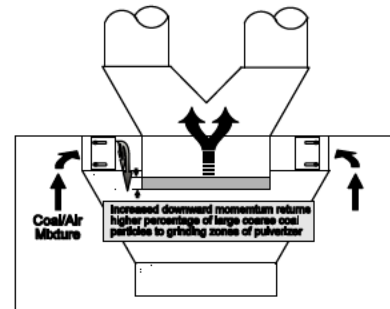
Figure 10 - Inverted Top Hat Extension
