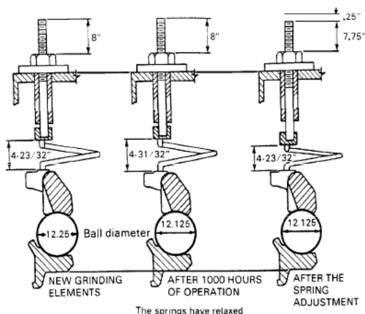
Figure 5 - Spring Adjustment by External Measurement
