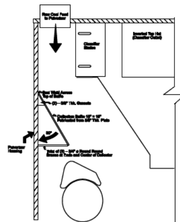
Figure 11 - Raw Coal Deflector for EL Pulverizers
