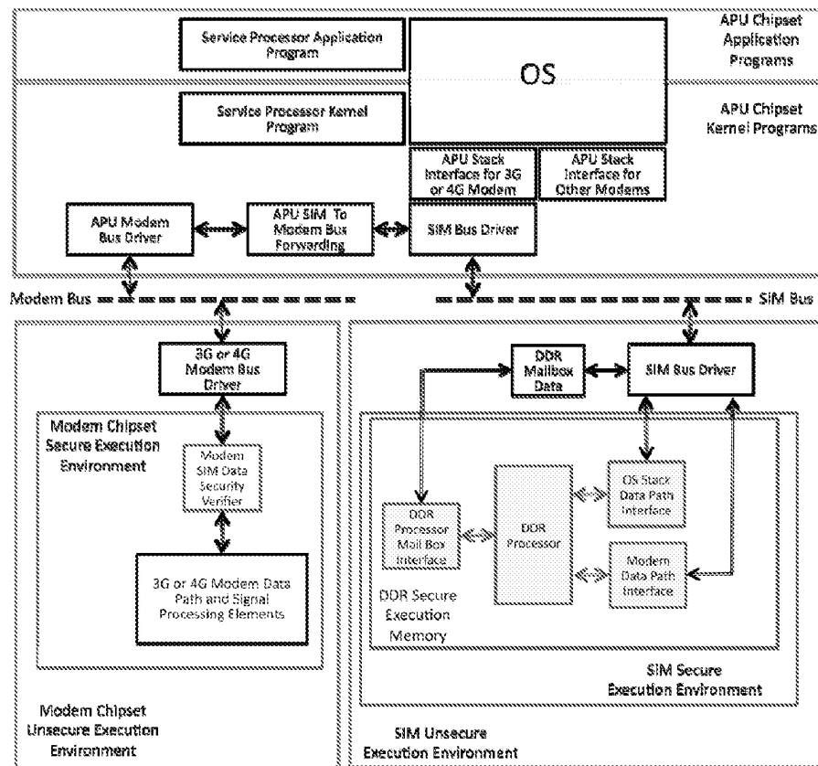
Figure 12: Details of Combined SIM DDR Processor and MPU Data Path Security Verifier
