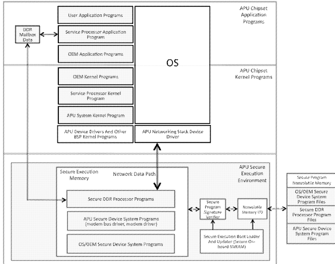
Figure 5: High Level Diagram of Secure Embedded DDR Processor in APU Implementation (option-1)
