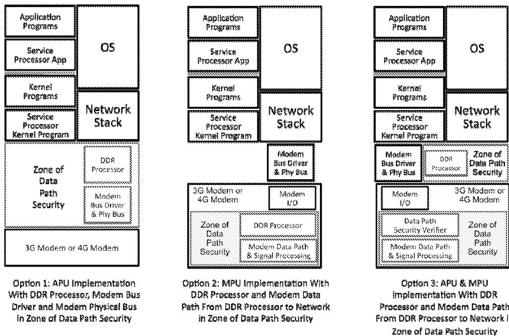
Figure 3: AWS Chipset Embedded DDR Processor Options
