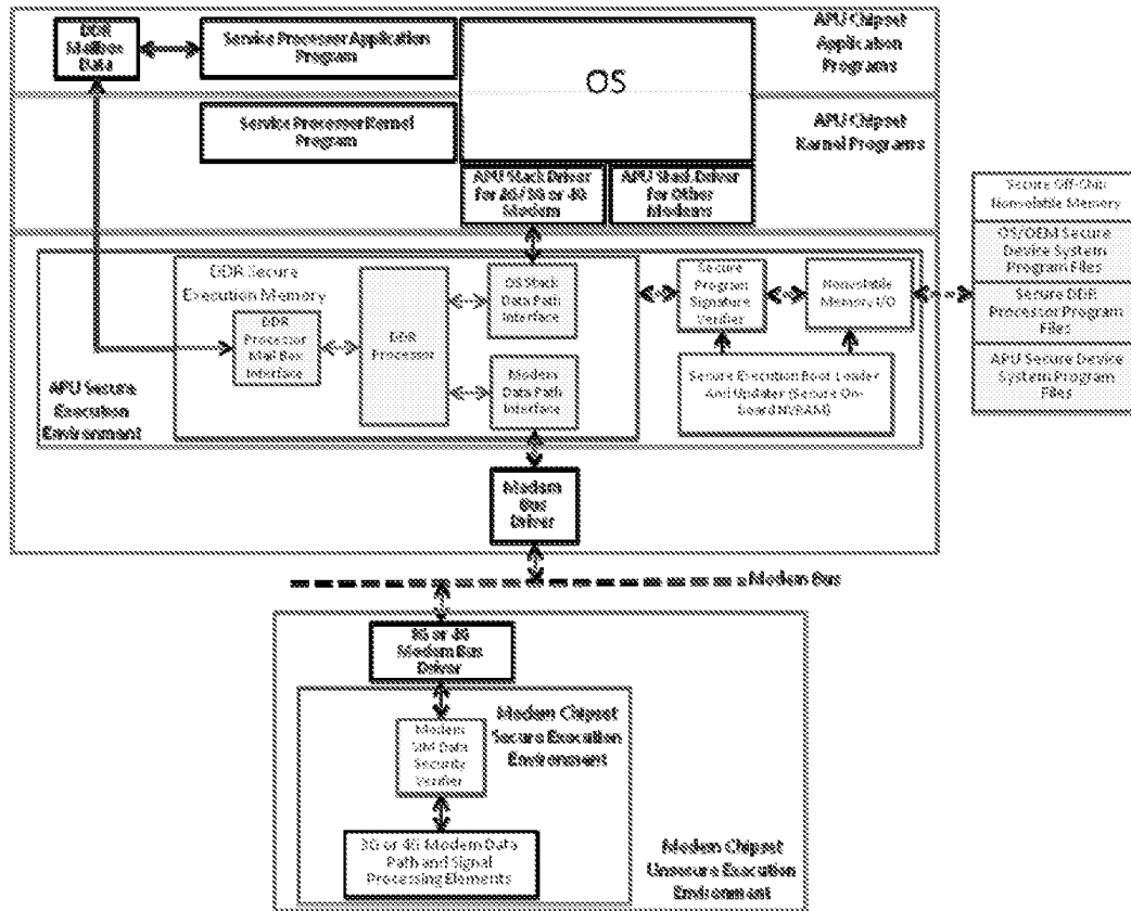
Figure 11: Details of Combined APU DDR Processor and MPU Data Path Security Verifier (option-3)
