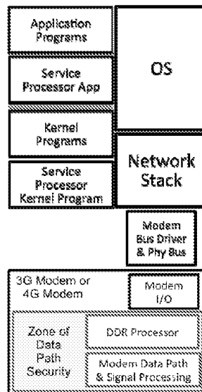
Figure 7: MPU Implementation (option-2) with Embedded DDR Processor and Modem Data Path From DDR Processor to Network in Zone of Data Path Security
