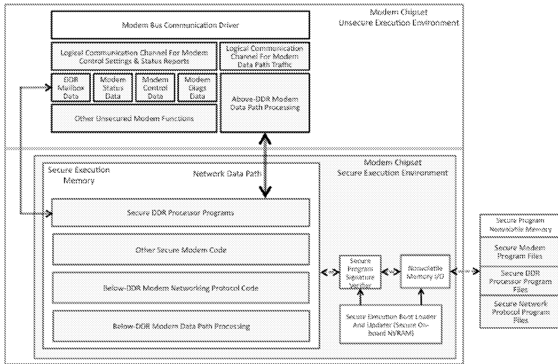
Figure 8: High Level Diagram of Embedded Secure DDR Processor in MPU Implementation (option-2)
