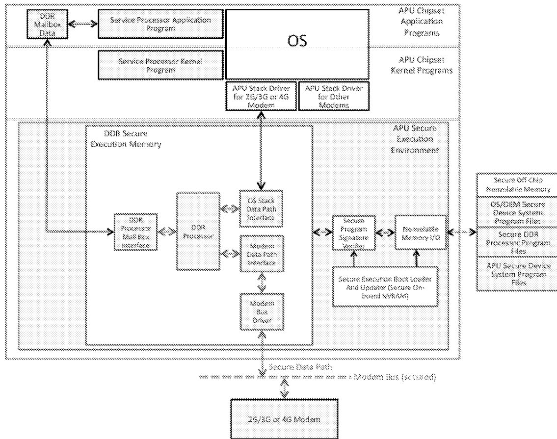
Figure 6: Details of Secure Embedded DDR Processor in SEE APU Implementation with Modem Bus Driver (option-1)
