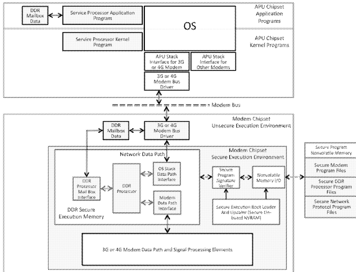
Figure 9: Details of Embedded Secure DDR Processor in SEE MPU Implementation (option-2)
