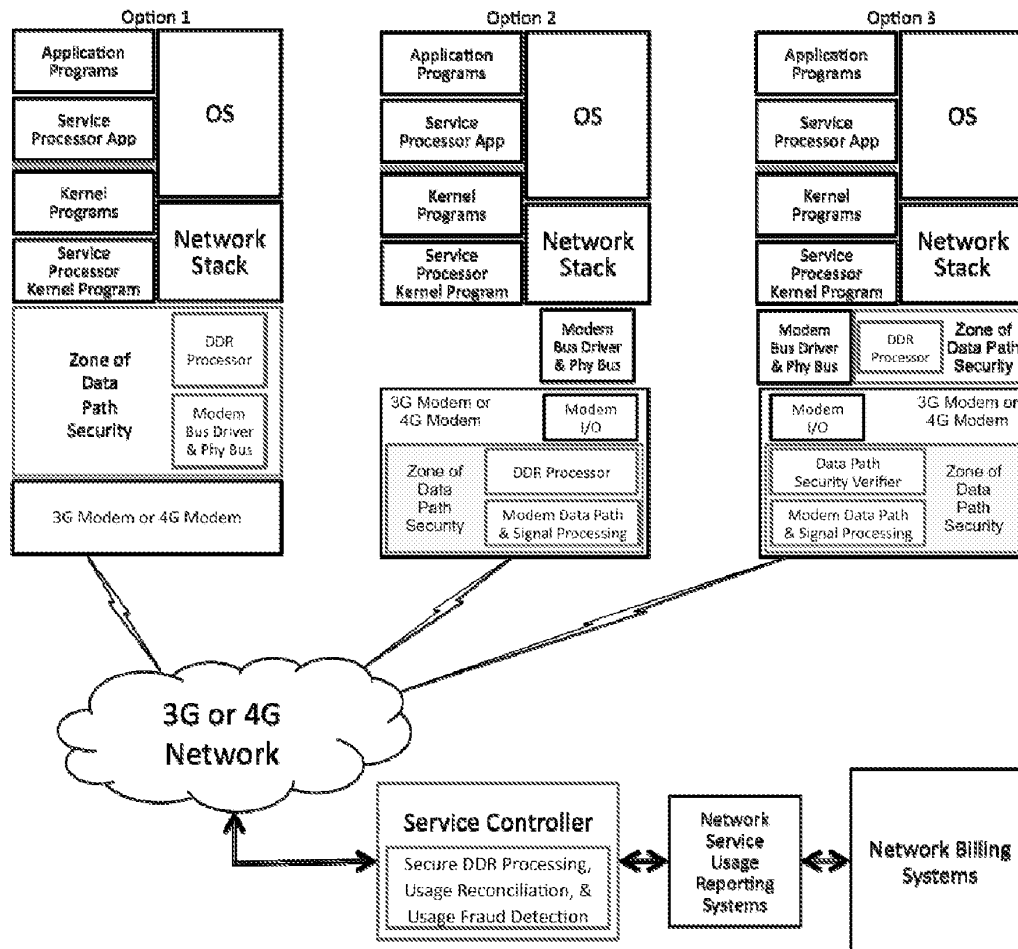
Figure 1: Advanced Wireless Service Platform End to End DDR Reporting and Processing System
