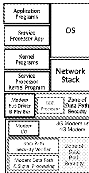
Figure 10: APU & MPU Implementation (option-3) with Embedded DDR Processor and Modem Data Path From DDR Processor to Network in Zone of Data Path Security
