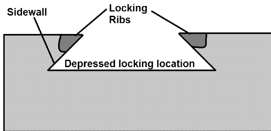
Diagram 3 - language of claim 9 as applied in a dovetail connection
