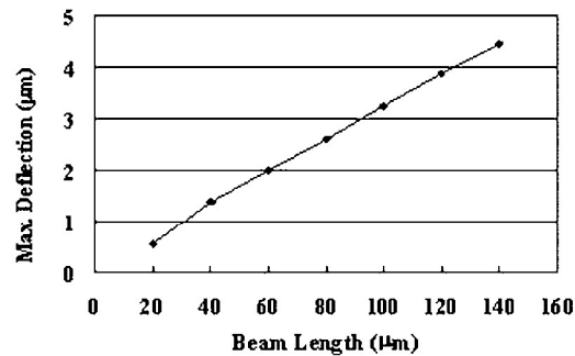
Fig. 6. Measured deflection amplitudes of \text{SiO}_2 microbridge vs beam length.
