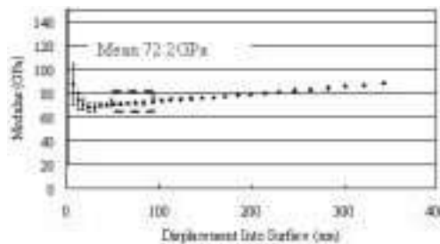
Fig. 3. Elastic moduli of thermal \text{SiO}_2 film at different indentation depths.
