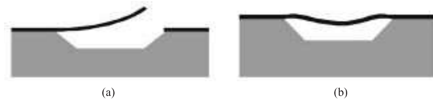
Fig. 2. Out-of-plane deformations: (a) microcantilever bending; and (b) microbridge buckling.
