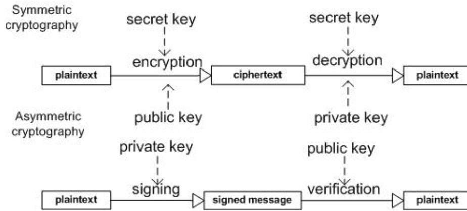
Figure 2.4: Symmetric and asymmetric cryptographical functions.
