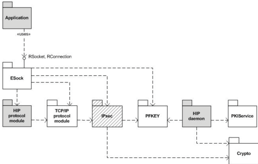
Figure 4.3: Package diagram of the core components related to HIP.
