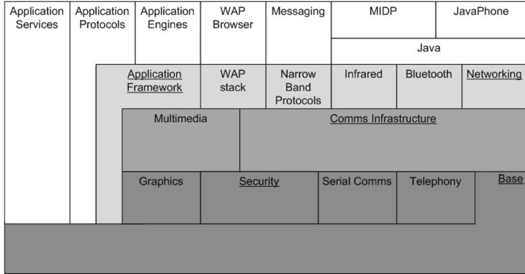
Figure 3.1: Symbian OS 9.2 is composed of several subsystems. [Sym06]
