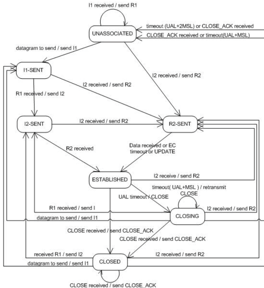
Figure 4.2: HIP state diagram
