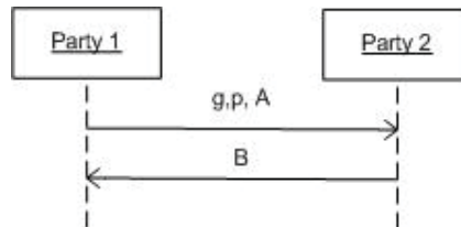
Figure 2.8: Diffie-Hellman key exchange.
