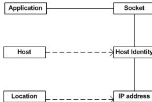
Figure 2.6: Logical entities connected to IP address along new Host Identity.
