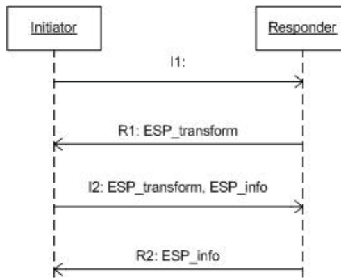
Figure 2.10: Setting up an ESP SA between HIP hosts during BEX
