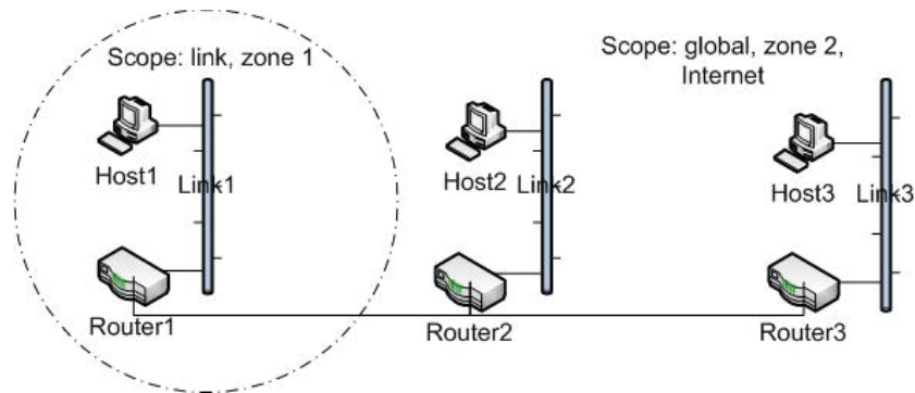
Figure 2.3: IPv6 address scopes.
