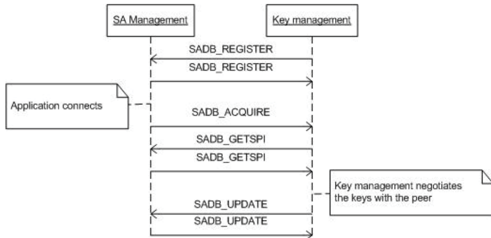
Figure 5.1: An example PFKEY message sequence for installing an SA.
