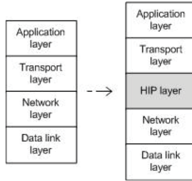
Figure 2.7: New stack architecture.
