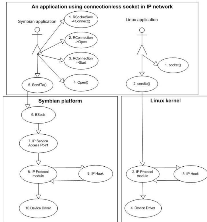
Figure 3.2: Connectionless socket send operation in Symbian and Linux.
