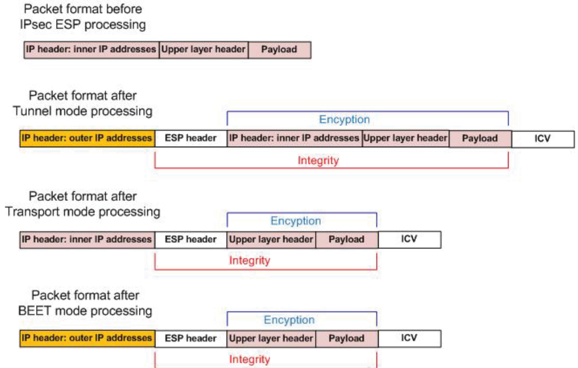
Figure 2.5: IPsec traffic modes and new mode BEET.
