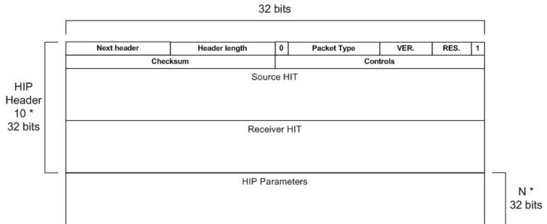
Figure 4.1: HIP PDU format.
