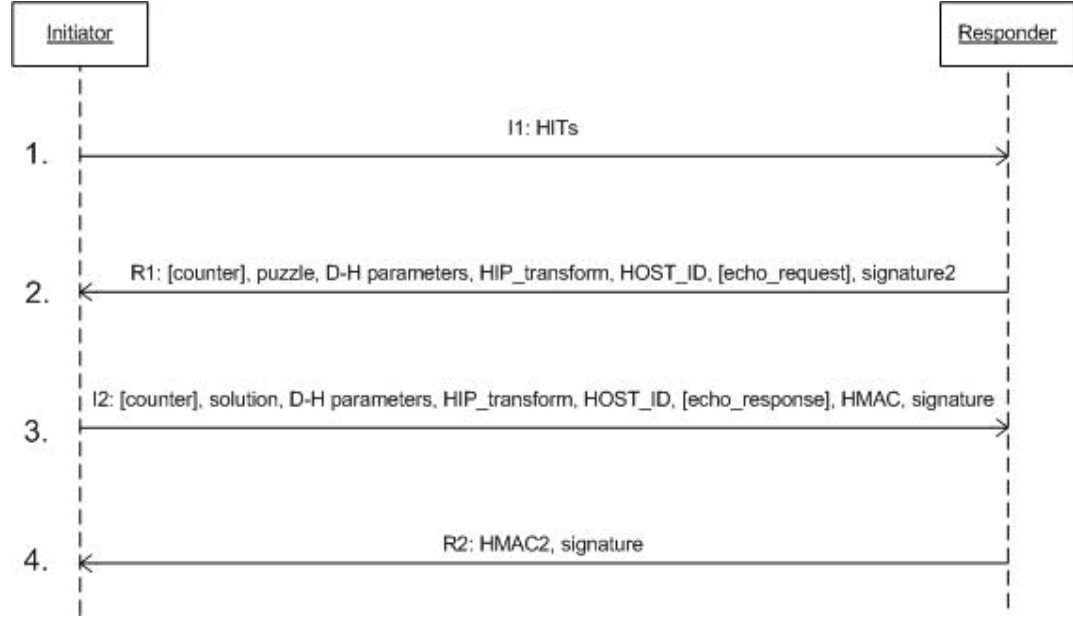
Figure 2.9: Host Identity Protocol Base Exchange.
