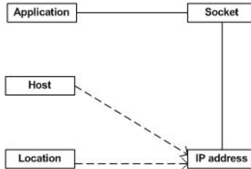
Figure 2.2: Logical entities connected to IP address.
