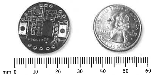
FIGURE 1-4. SkyeTek's SkyeRead M1-mini (image courtesy of SkyeTek)
