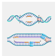
DNA Replication
