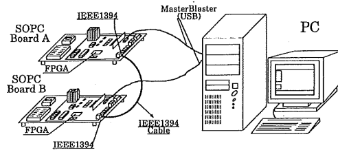
Fig. 6 System used for experiment (1).
