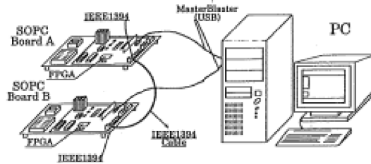
Fig. 6 System used for experiment (1).
