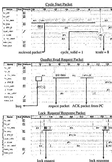
Fig. 10 Waveforms observed at SOPC board in experiment (2).
