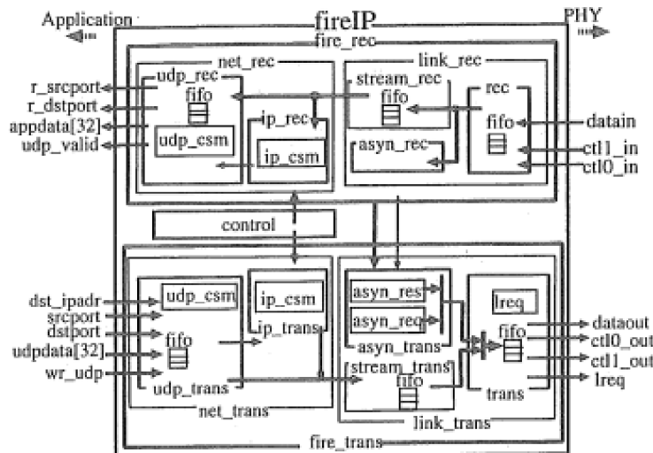
Fig. 5 Block diagram of fireIP module.
