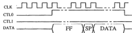
Fig. 3 Receive operation.
