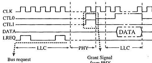
Fig. 2 Transmit operation.
