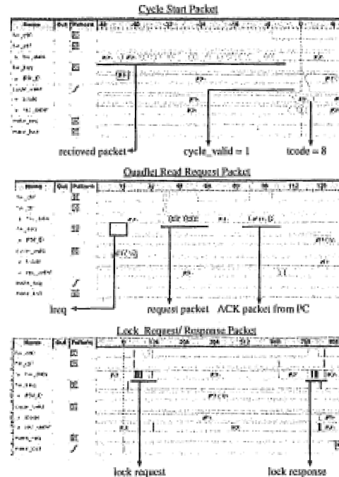
Fig. 10 Waveforms observed at SOPC board in experiment (2).
