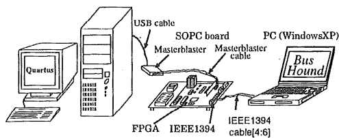
Fig. 9 System used for experiment (2).
