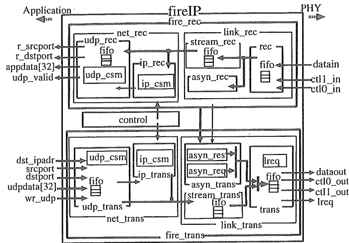
Fig. 5 Block diagram of fireIP module.
