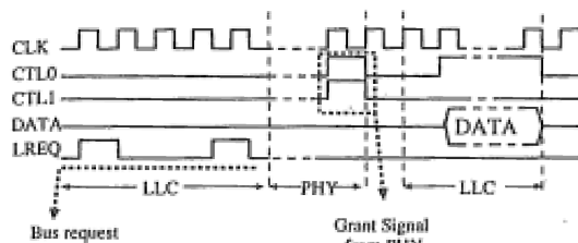
Fig. 2 Transmit operation.
