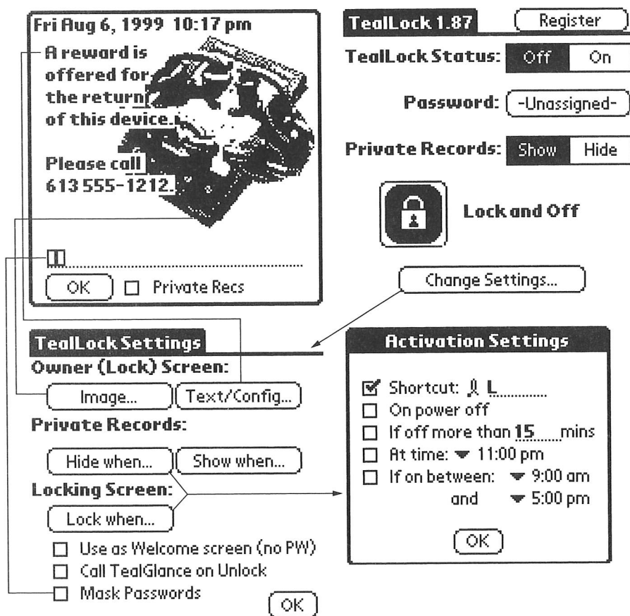
Figure 21-26: TealLock settings
