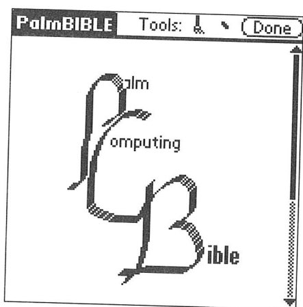
Figure 17-7: SimpleSketch
