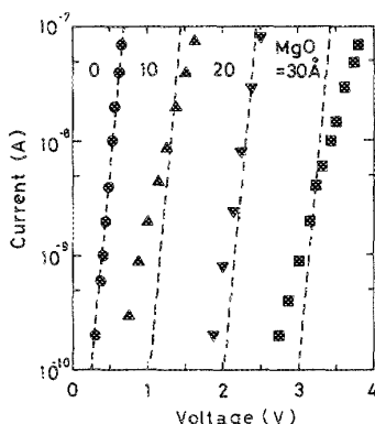
FIG. 9. Current-voltage curves of the prepared MIS tunneling Schottky diode as a parameter of the MgO thickness.
