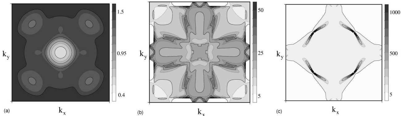
FIG. 4. (a) The smallest decay constant \text{Im } k_{\perp}(\mathbf{k}_{\parallel}) of electrons in the MgO barrier (the lowest sheet of the complex MgO Fermi surface). (b) The majority-spin surface spectral density of Fe(001). (c) The minority-spin surface spectral density of Fe(001).
