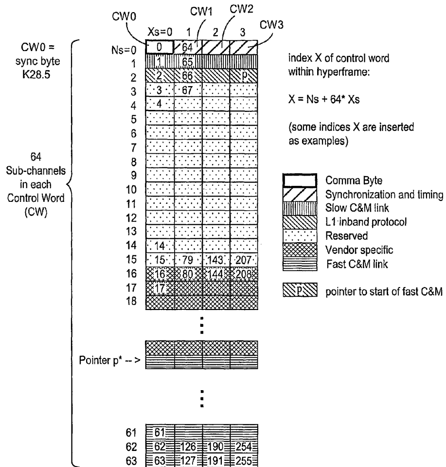
Illustration of subchannels within one hyperframe
