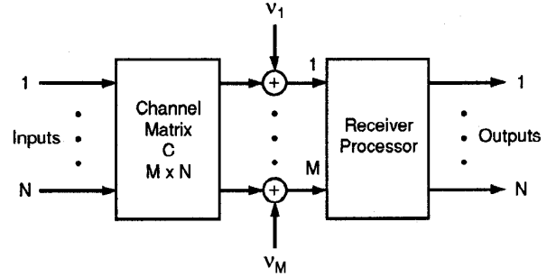
Fig. 1. Multiuser communication block diagram.
