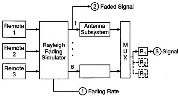
Fig. 4. Experimental system.
