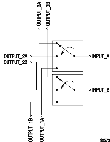
Figure 1. SKY13399-468LF Block Diagram
