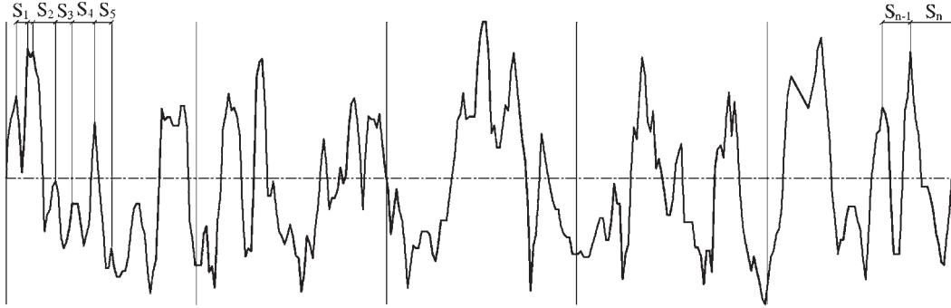
Fig. 11. Calculating the mean spacing of adjacent local peaks ( S ).
