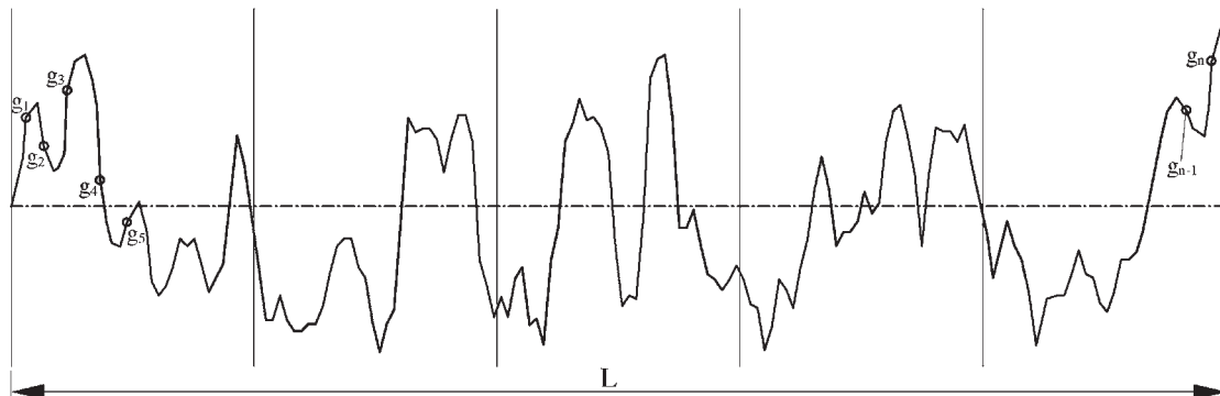
Fig. 15. Calculating the number of inflection points along the profile.
