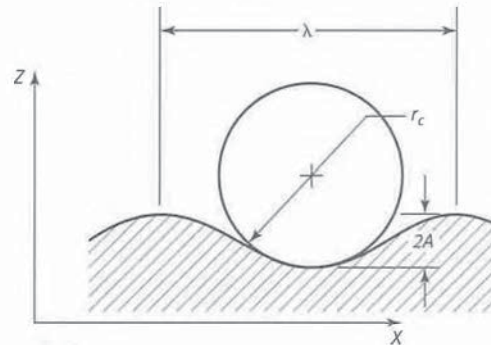
Fig. 7-1 The Radius of Curvature for a Surface Sine Wave
