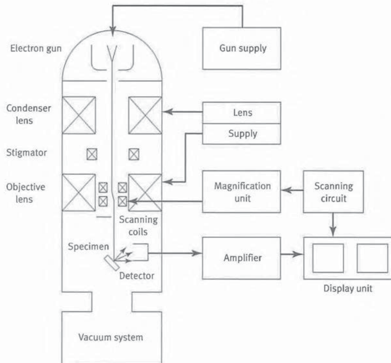
Fig. C-9 Diagram of Scanning Electron Microscope
