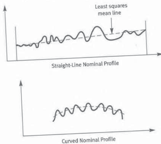
Fig. 1-4 Examples of Nominal Profiles
