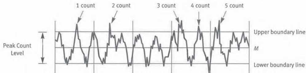
Fig. 1-14 The Peak Count Level, Used for Calculating Peak Density
