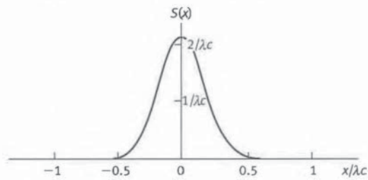
Fig. 9-3 Weighting Function of the Gaussian Profile Filter (This material is produced from ISO 11562:1996.)
