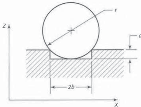
Fig. 7-2 Stylus Tip Touching Bottom and Shoulders of Groove
