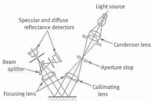
Fig. C-2 Reflectance Measurement
