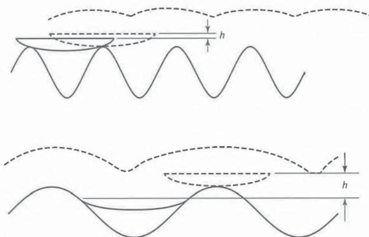
Fig. 4-3 Examples of Profile Distortion Due to Skid Motion
