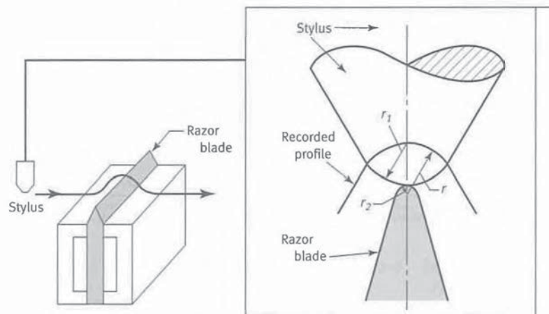
Fig. 11-7 Use of Type B3 Specimen
