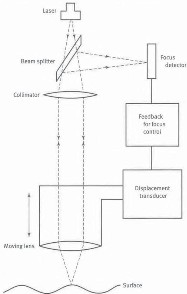
Fig. E-1 Schematic Diagram of an Optical Focus-Sensing Instrument
