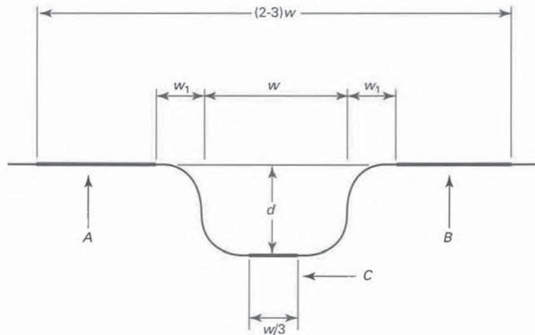
Fig. 11-4 Assessment of Calibrated Values for Type A1
