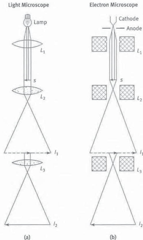
Fig. C-8 Comparison of Optical and Transmission Electron Microscope
