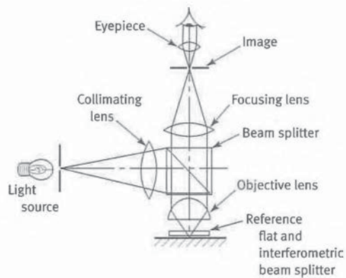
Fig. C-4 Multiple Beam Interferometer
