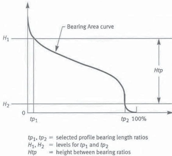
Fig. 1-17 The Bearing Area Curve and Related Parameters
