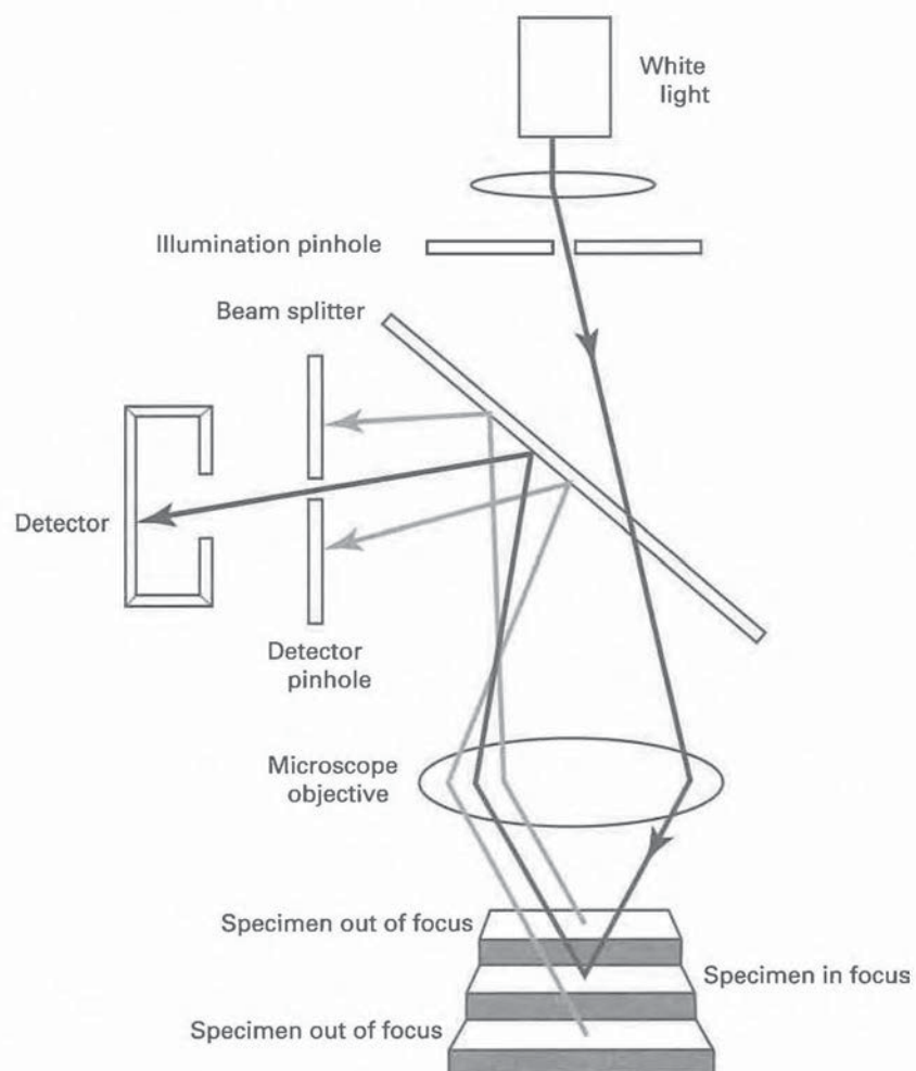
Fig. E-6 Schematic Diagram of a Confocal Microscope
