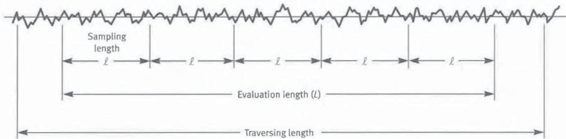
Fig. 1-7 Surface Profile Measurement Lengths
