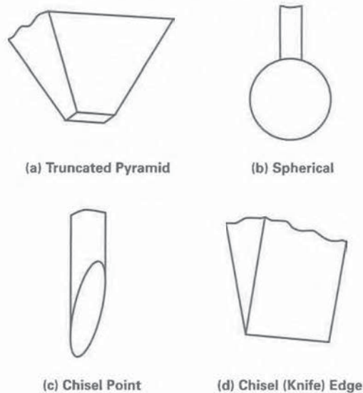
Fig. 3-3 Other Stylus Tip Geometries
