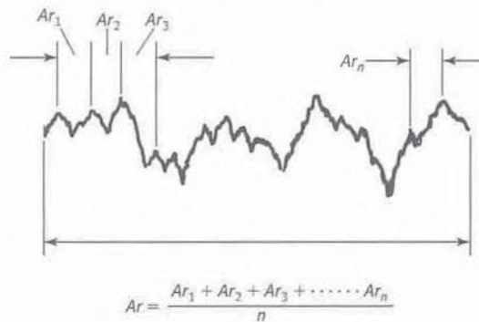
Fig. D-2 Average Spacing of Roughness Peaks
