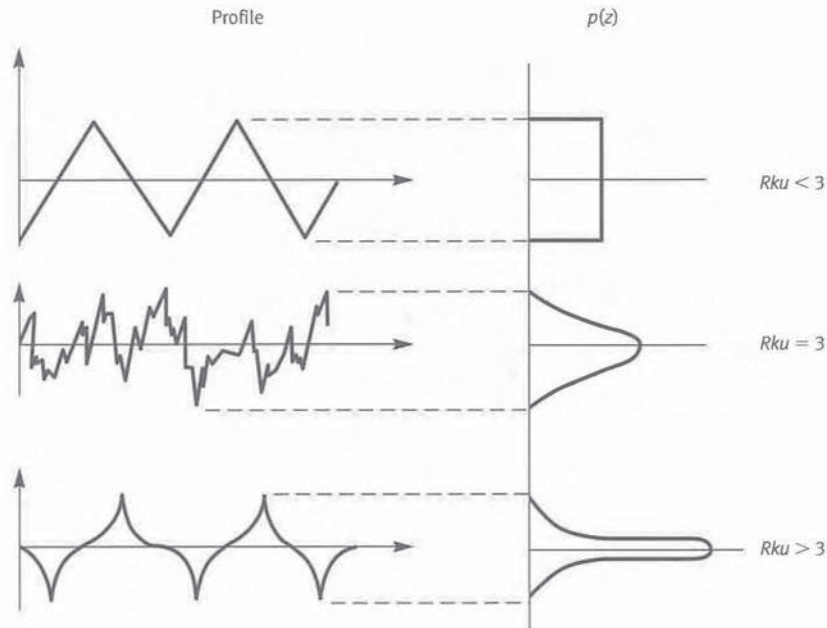
Fig. 1-19 Three Surface Profiles With Different Kurtosis
