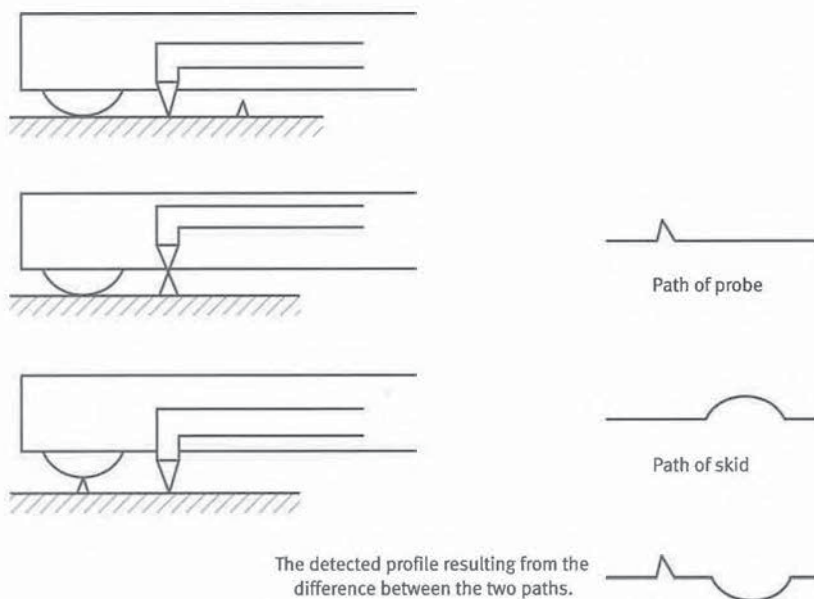
Fig. 4-4 Examples of Profile Distortion
