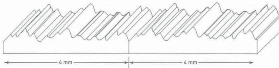
Fig. 11-11 Unidirectional Irregular Groove Specimen Having Profile Repetition at 5\lambda c Intervals (Type D1 With \lambda c = 0.8 mm)
