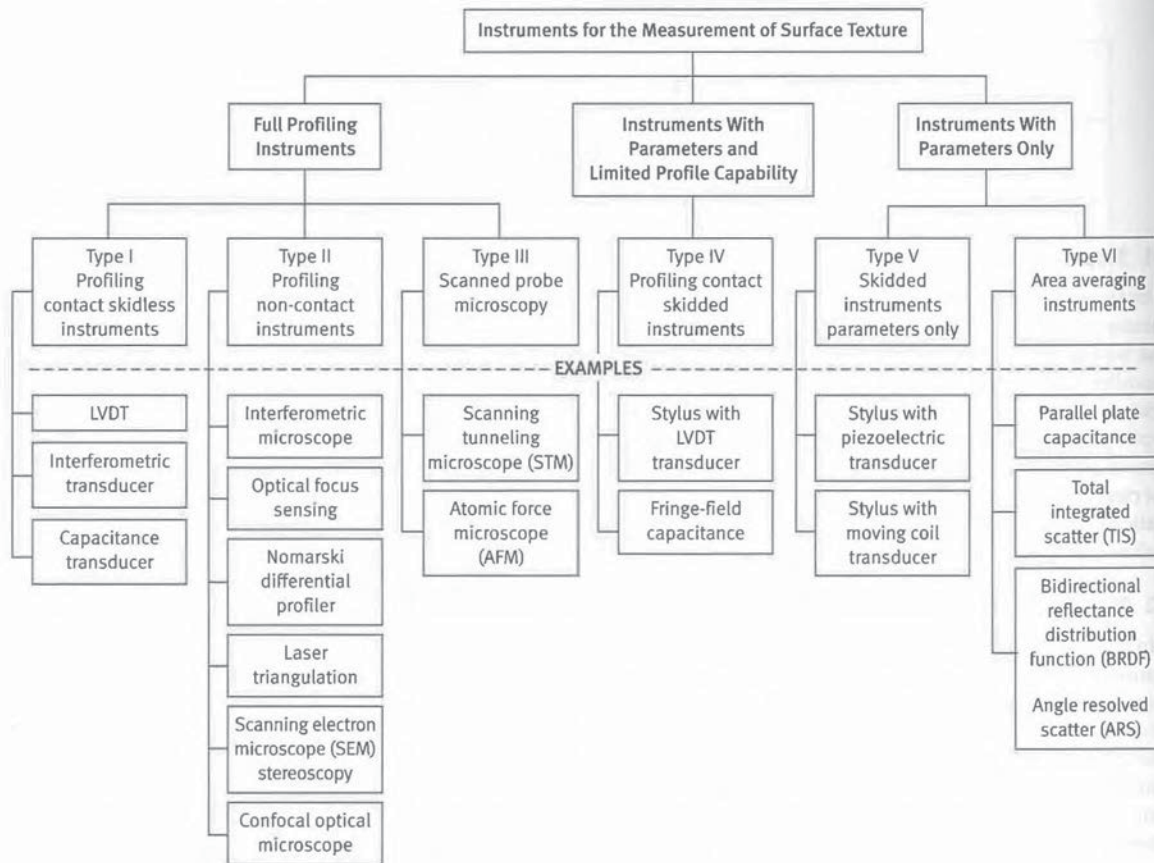
Fig. 2-1 Classification of Common Instruments for Measurement of Surface Texture
