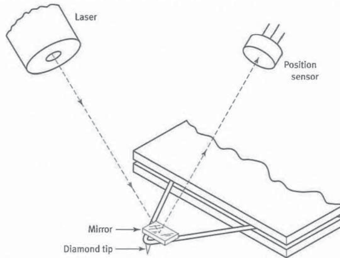
Fig. E-5 Schematic Diagram of an Atomic Force Microscope With an Optical Lever Sensor
