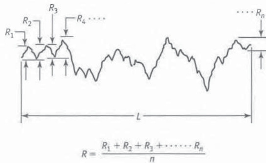
Fig. D-1 Average Peak-to-Valley Roughness
