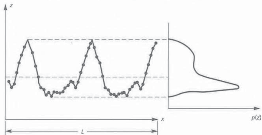
Fig. 1-15 Amplitude Density Function — ADF(z) or p(z)
