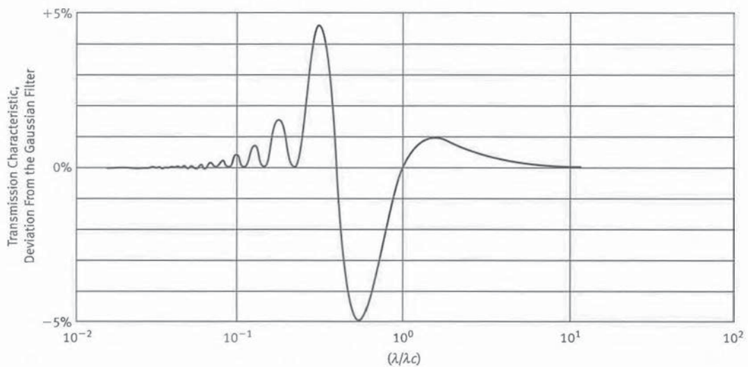
Fig. 9-6 Example of a Deviation Curve of an Implemented Filter From the Ideal Gaussian Filter as a Function of Spatial Wavelength (This material is produced from ISO 11562:1996.)
