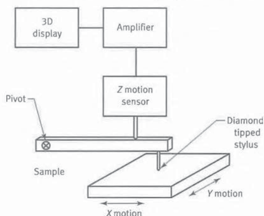
Fig. E-3 Area Scanning Stylus Profiler
