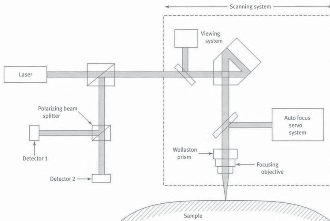
Fig. E-2 Schematic Diagram of Nomarski Differential Profiler
