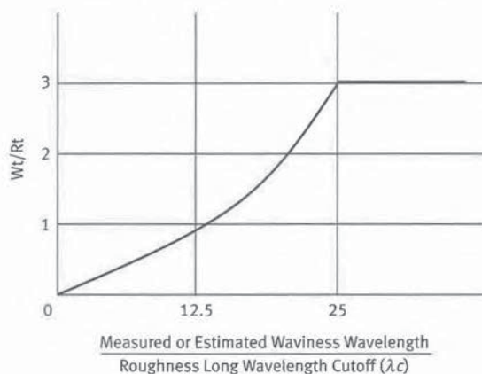
Fig. 11-3 Allowable Waviness Height Wt for Roughness Calibration Specimens
