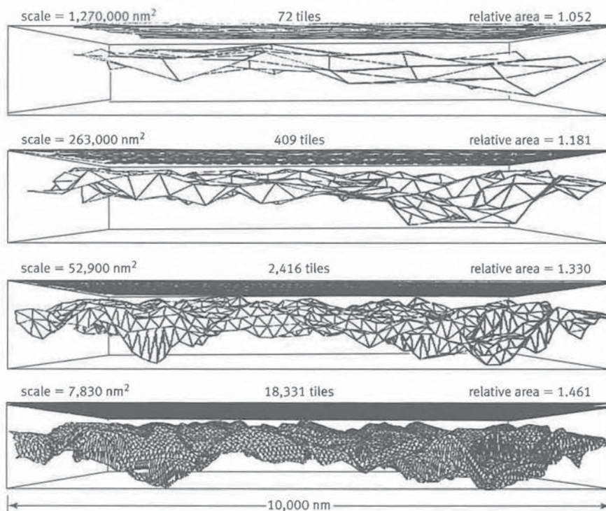
Fig. 10-5 Four Tiling Exercises From an Area-Scale Analysis
