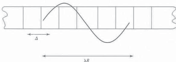
Fig. 8-3 Demonstration of the Detector Array With Element Spacing \Delta and the Measurement of the Smallest Spatial Wavelength, \lambda R Covering Five Pixels
