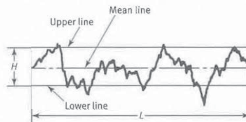
Fig. D-3 Swedish Height of Irregularities
