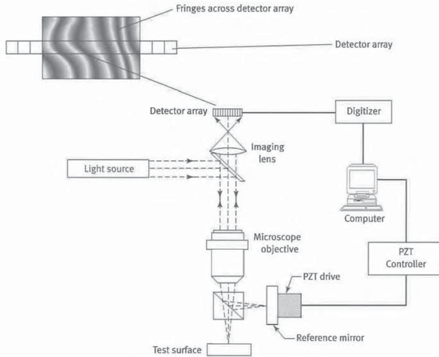
Fig. 8-1 A Typical Phase Measuring Interferometer System
