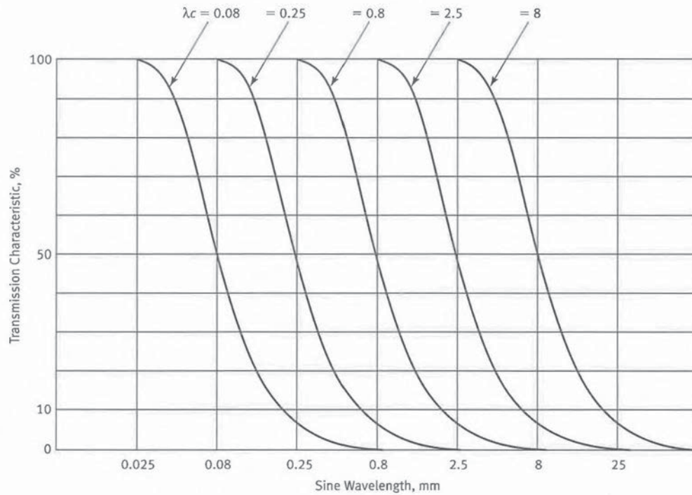
Fig. 9-5 Gaussian Transmission Characteristic for the Roughness Long-Wavelength Cutoff Having Cutoff Wavelengths \lambda_c = 0.08 mm, 0.25 mm, 0.8 mm, 2.5 mm, and 8.0 mm (This material is produced from ISO 11562:1996.)
