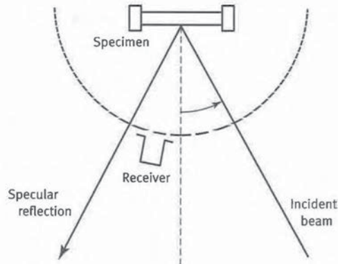
Fig. F-4 Schematic Diagram of an Instrument for Measuring ARS or BRDF
