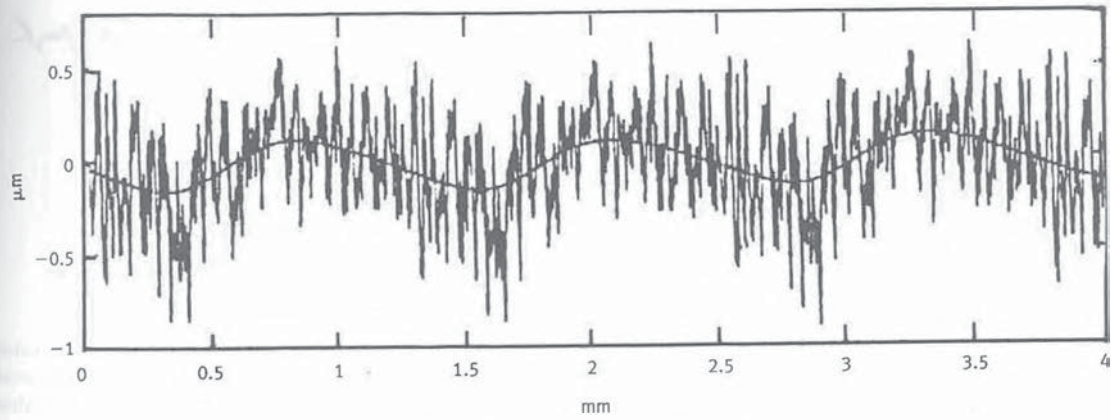
(a) Unfiltered Profile and Filtered Mean Line
