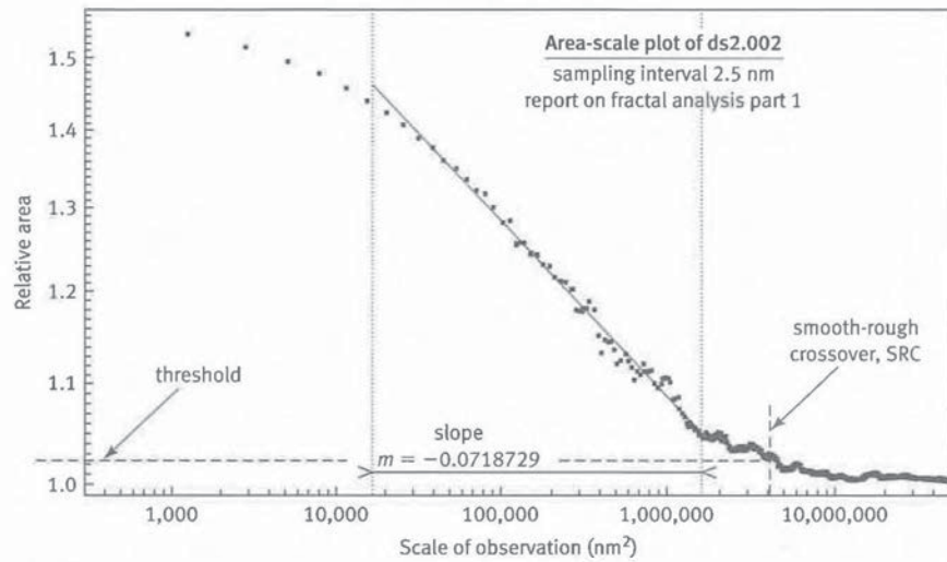
Fig. 10-6 An Area-Scale Plot Including the Results of the Tiling Series in Fig. 10-5
