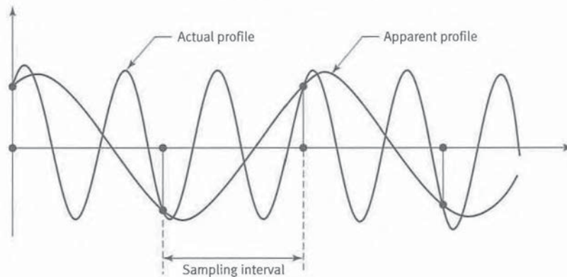
Fig. 3-4 Aliasing
