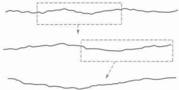
Fig. 10-1 Self-Similarity Illustrated on a Simulated Profile
