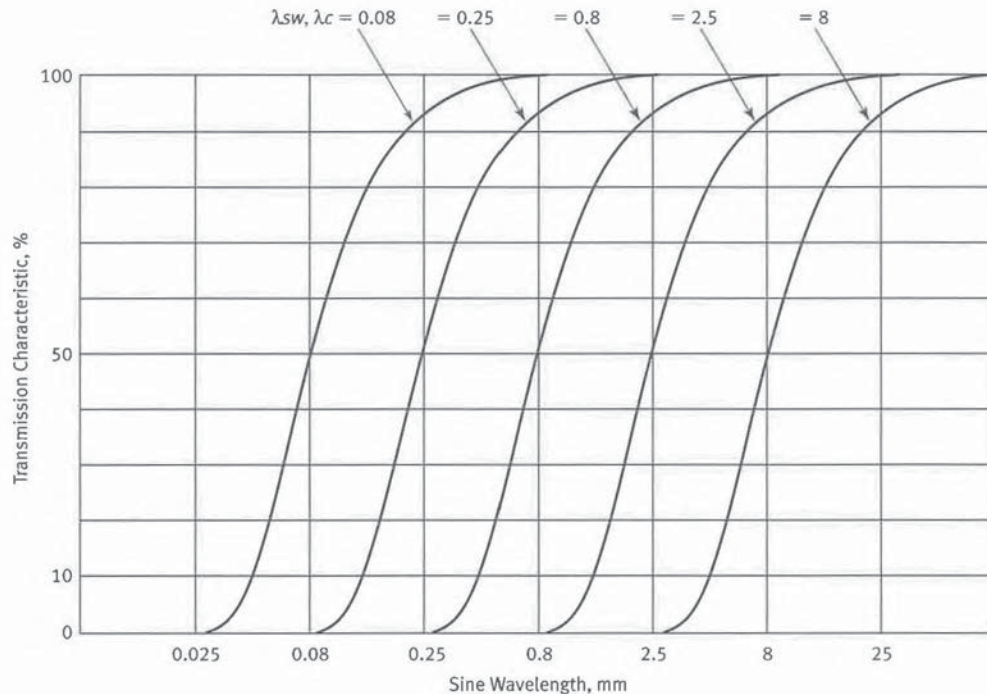
Fig. 9-4 Gaussian Transmission Characteristic for the Waviness Short-Wavelength Cutoff ( \lambda_{sw} ) or for Deriving the Roughness Mean Line Having Cutoff Wavelengths ( \lambda_c ) of 0.08 mm, 0.25 mm, 0.8 mm, 2.5 mm, and 8.0 mm
