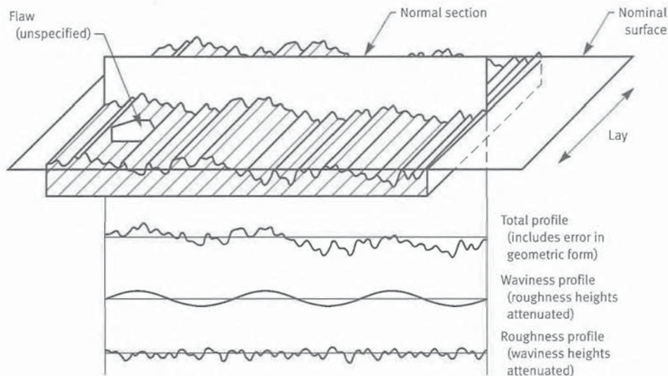
Fig. 1-1 Schematic Diagram of Surface Characteristics
