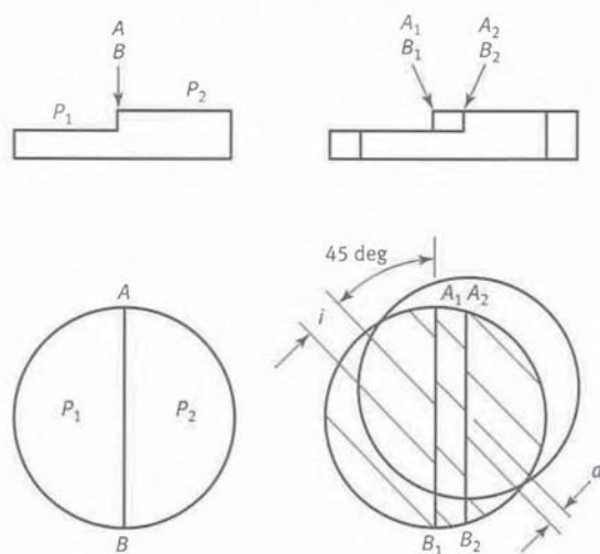
Fig. C-6 Differential Interferometry
