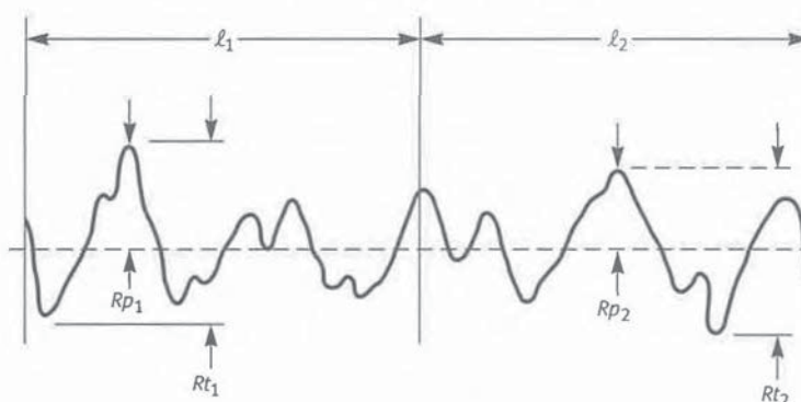
Fig. 1-10 Surface Profile Containing Two Sampling Lengths, l_1 and l_2 , Also Showing the R_{p_i} and R_{t_i} Parameters
