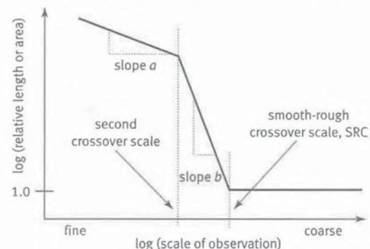
Fig. 10-3 An Idealized Log-Log Plot of Relative Length or Area Versus the Scale of Observation (Length-Scale or Area-Scale Plot), Showing Multi-Fractal Characteristics and Crossover Scales
