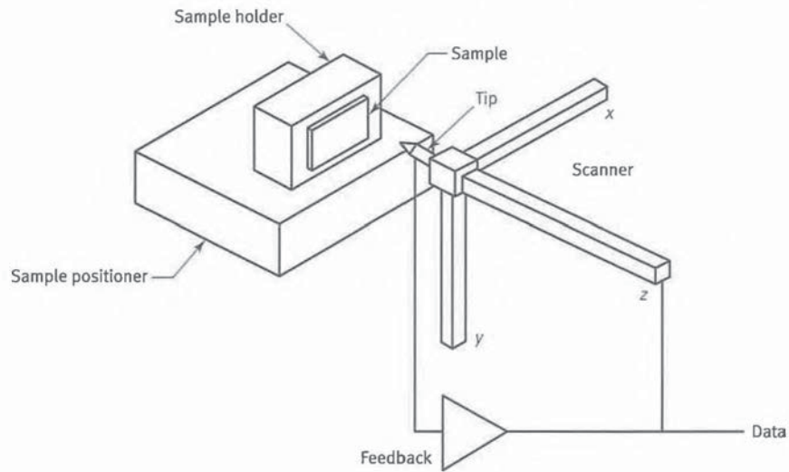
Fig. E-4 Basic Structure of an Early STM
