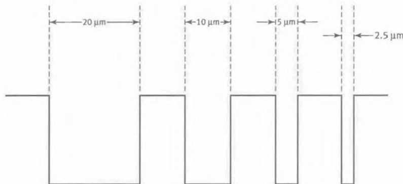
Fig. 11-5 Type B1 Grooves: Set of Four Grooves
