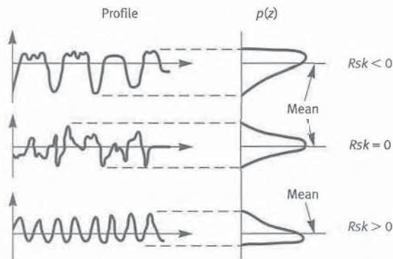
Fig. 1-18 Three Surface Profiles With Different Skewness
