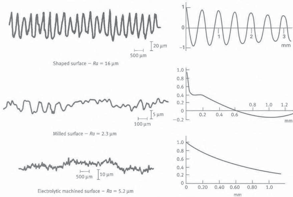
Fig. D-4 Measured Profiles and Their Autocorrelation Functions
