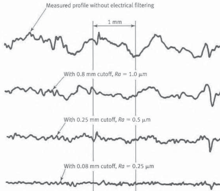
Fig. 4-2 Effects of Various Cutoff Values
