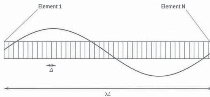
Fig. 8-2 Demonstration of the Detector Array With Element Spacing \Delta and the Measurement of the Longest Spatial Wavelength, \lambda L Covering the Total Number ( N ) Pixels
