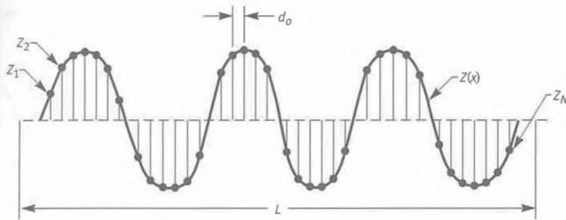
Fig. 1-8 Illustration for the Calculation of Roughness Average R_a
