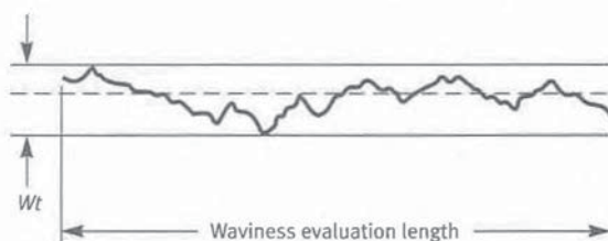
Fig. 1-12 The Waviness Height, W_t
