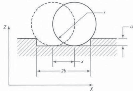
Fig. 7-3 The Stylus Tip Contact Distance, x
