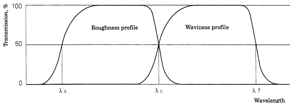
Figure 1 Transmission characteristic of roughness and waviness profiles
