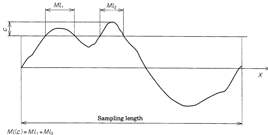
Figure 5 Material length
