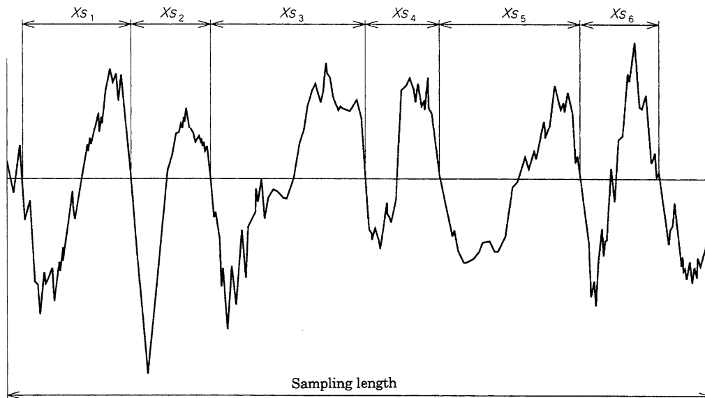
Figure 10 Width of profile elements
