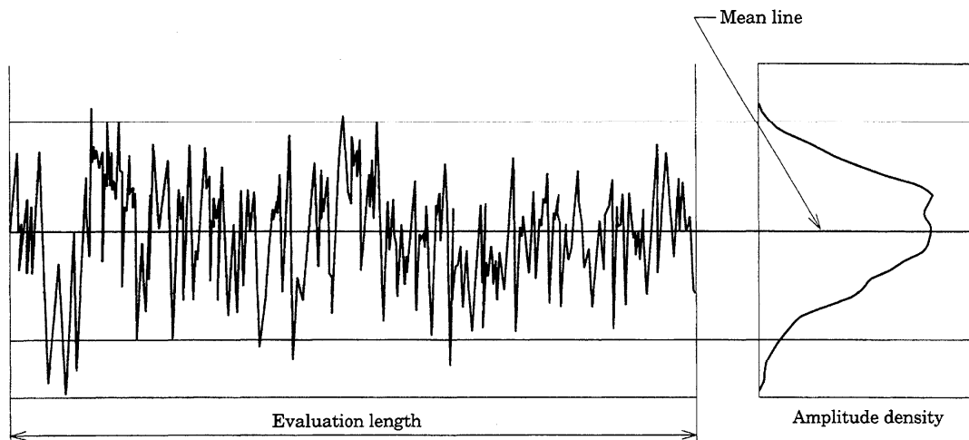
Figure 13 Profile height amplitude distribution curve
