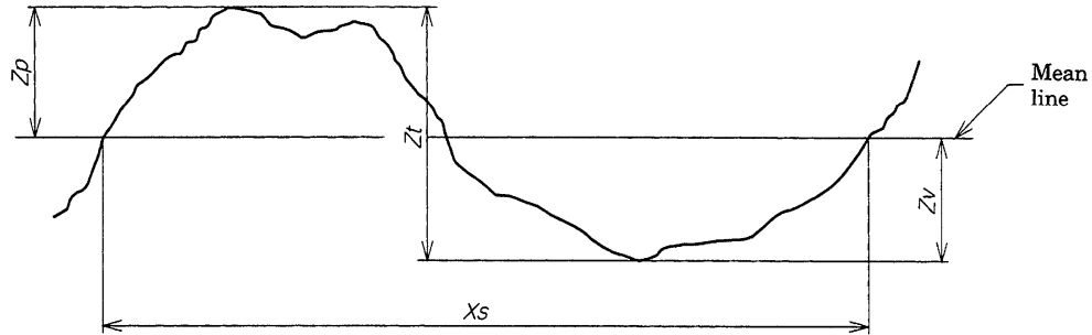
Figure 3 Profile element
