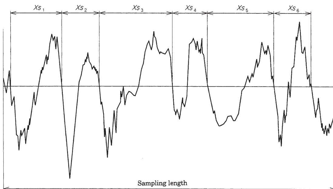
Figure 10 Width of profile elements
