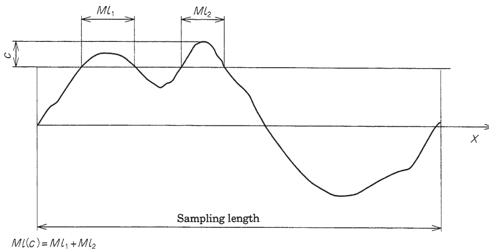
Figure 5 Material length
