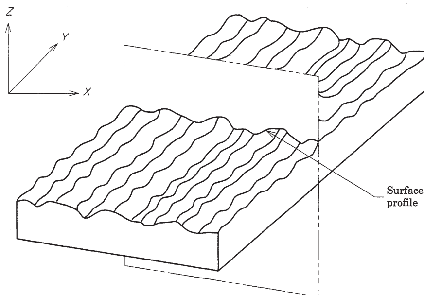
Figure 2 Surface profile
