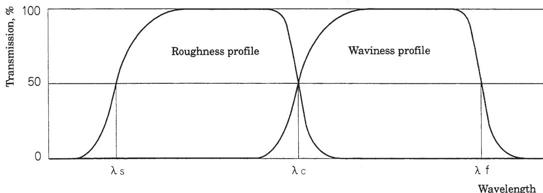
Figure 1 Transmission characteristic of roughness and waviness profiles
