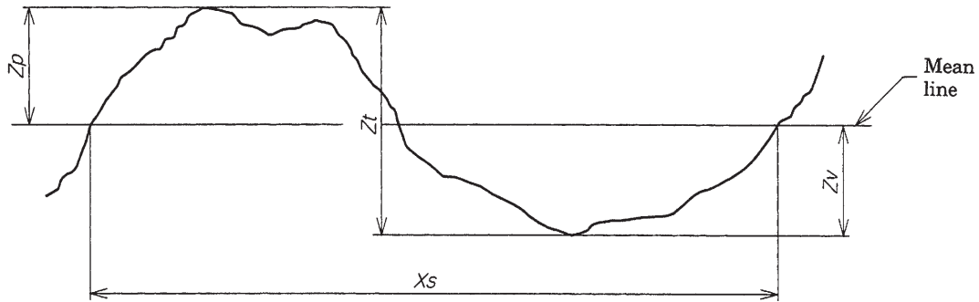
Figure 3 Profile element
