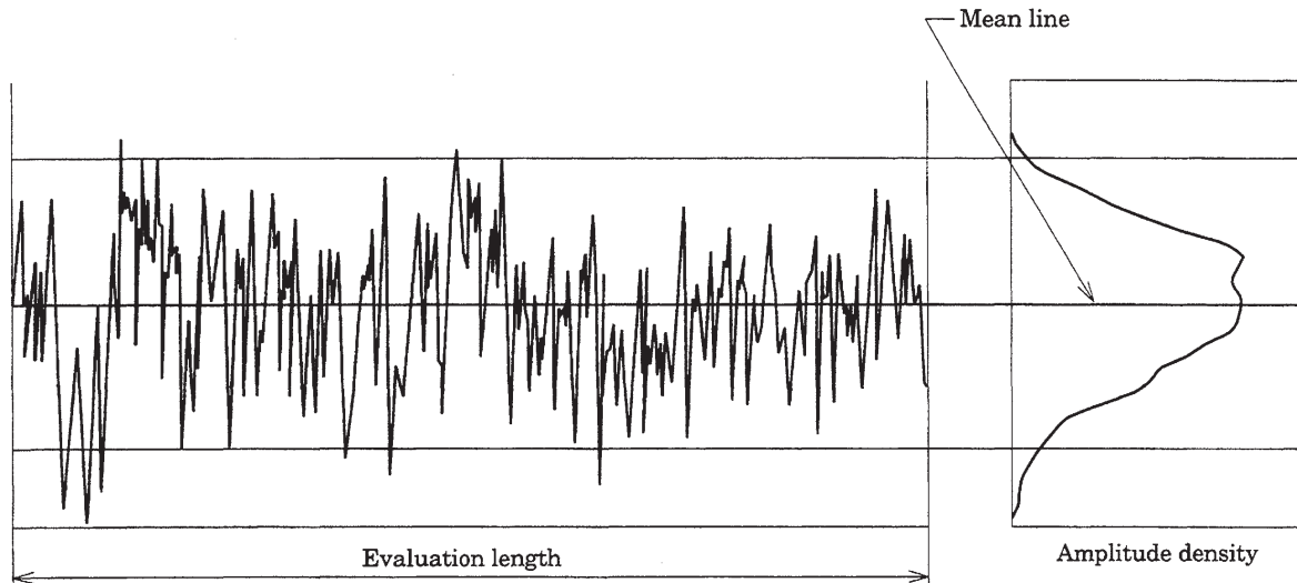
Figure 13 Profile height amplitude distribution curve
