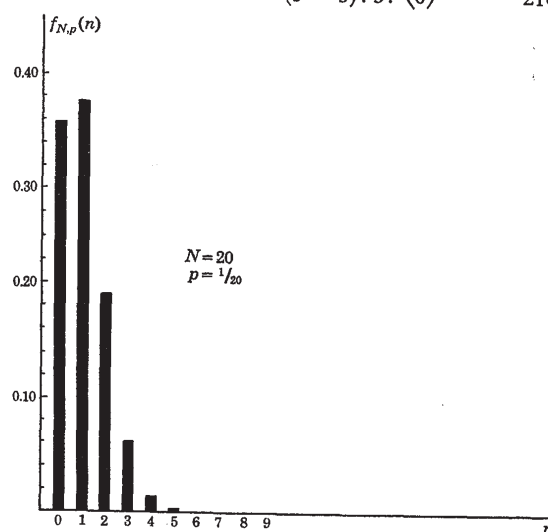
Fig. 7.2c. Example of binomial distribution, with N = 20 . Distribution is strongly asymmetric. Here \bar{n} = 1 , and probabilities for n > 6 are negligibly small.
