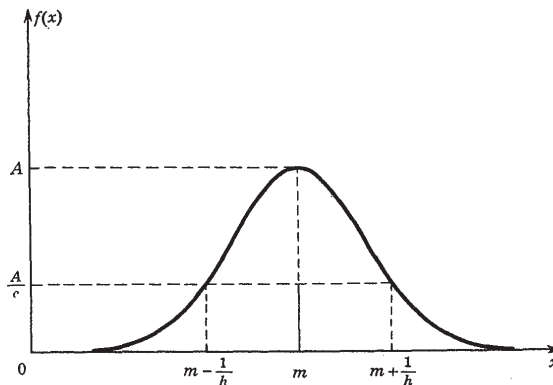
Fig. 9.1. Gauss distribution function. The points x = m \pm 1/h , at which the curve has 1/e of its maximum height, are shown.
