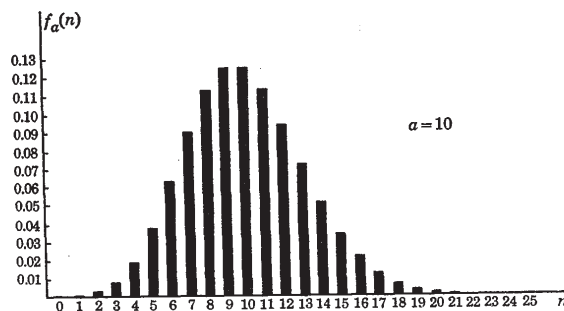
Fig. 8.2. Poisson distribution with a = 10 .
