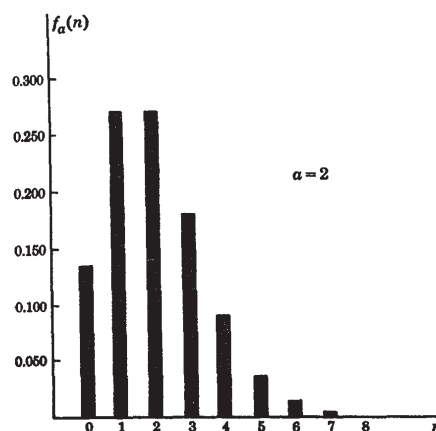
Fig. 8.1. Poisson distribution with a = 2 .
