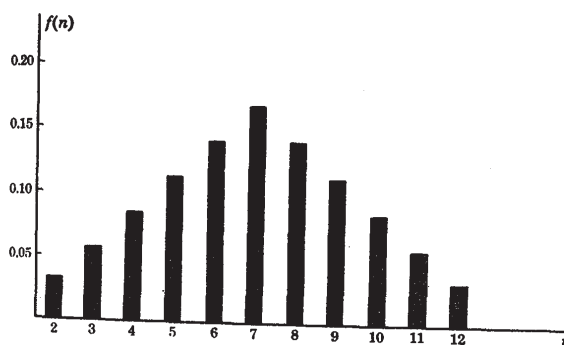
Fig. 6.1. Probability distribution for two dice.
