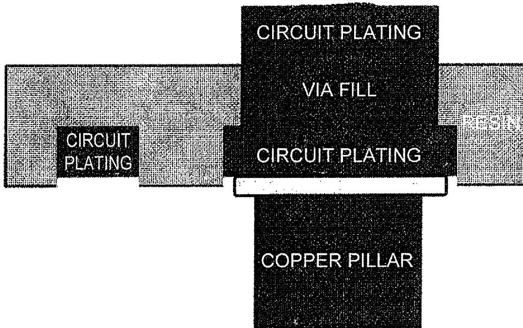
BUMP AND COPPER PILLAR FORMATION
