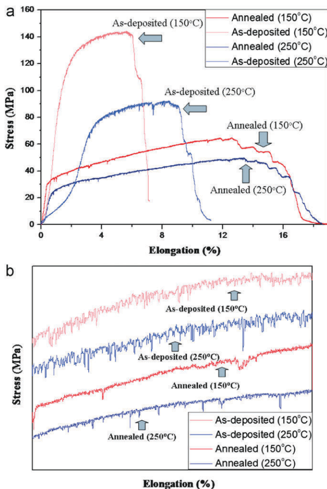
Fig. 15. (a) Tensile stress and strain curves of as-deposited and annealed VLP-D samples, and (b) serrate flows on enlarged curves.
