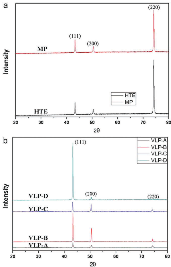
Fig. 3. X-ray diffraction patterns of the Cu foils: (a) HTE and MP, (b) VLP series.
