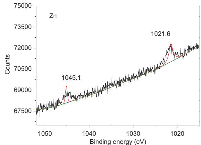
Fig. 8. Zn2p signal on the XPS spectrum for the VLP-B samples.
