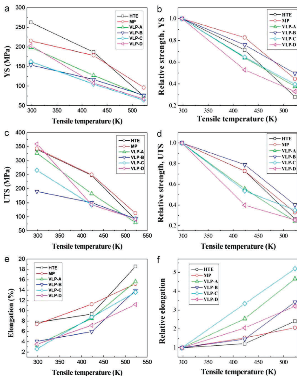
Fig. 14. Variation in tensile properties and their relative values with respect to test temperature: (a and b) yield strength, (c and d) ultimate tensile strength and (e and f) elongation gain.
