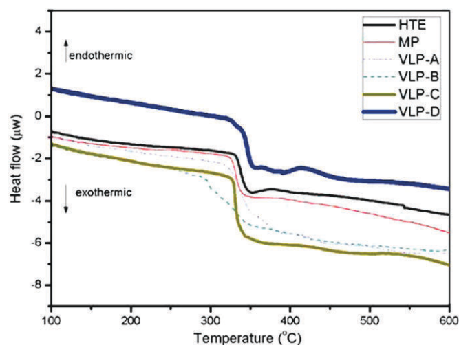
Fig. 9. DSC curves upon heating.
