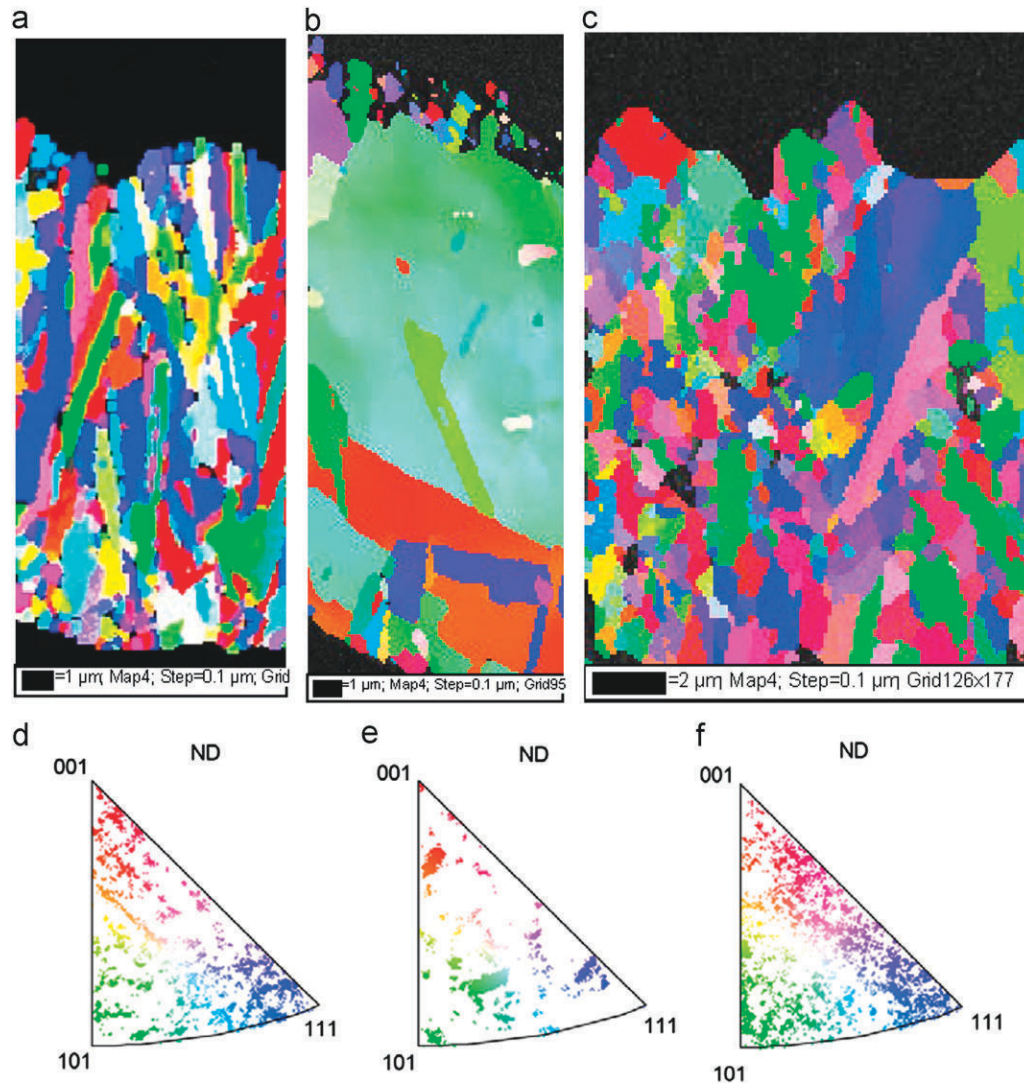
Fig. 7. EBSD images and inverse pole figures of the selected Cu foils: (a and d) HTE ((220)), (b and e) VLP-C ((200)) and (c and f) VLP-D ((111)) (ND: normal direction to the cross-sectioned plane).
