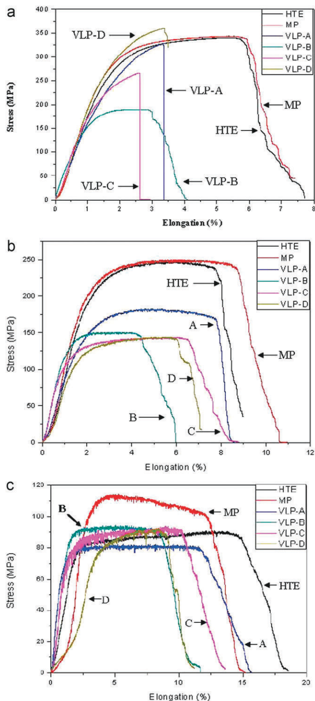
Fig. 11. Tensile stress-strain curves at different testing temperatures: (a) room temperature, (b) 150 °C and (c) 250 °C.
