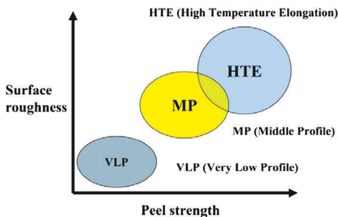
Fig. 2. Properties of commercial Cu foils for PCB applications.
