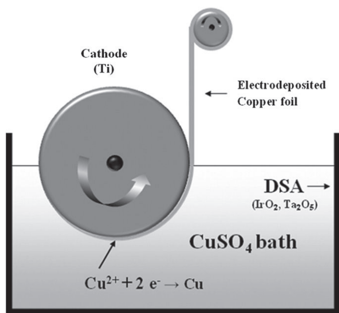
Fig. 1. Schematic diagram of the electroplating process for Cu foils (DSA: dimensional stable anode).
