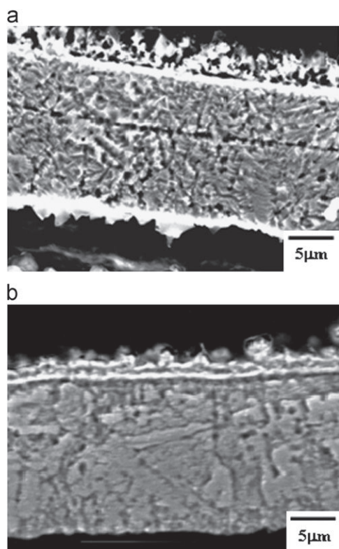
Fig. 5. Cross-sectional microstructure of (200) oriented foils (a) VLP-B and (b) VLP-C.
