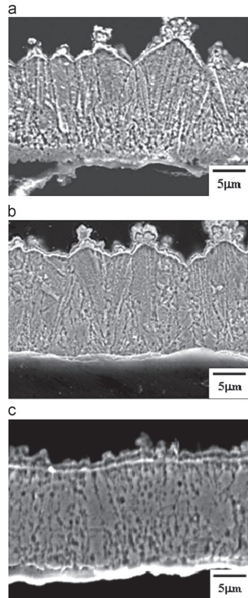
Fig. 4. Cross-sectional microstructure of (220) oriented foils (a) HTE, (b) MP and (c) VLP-A.
