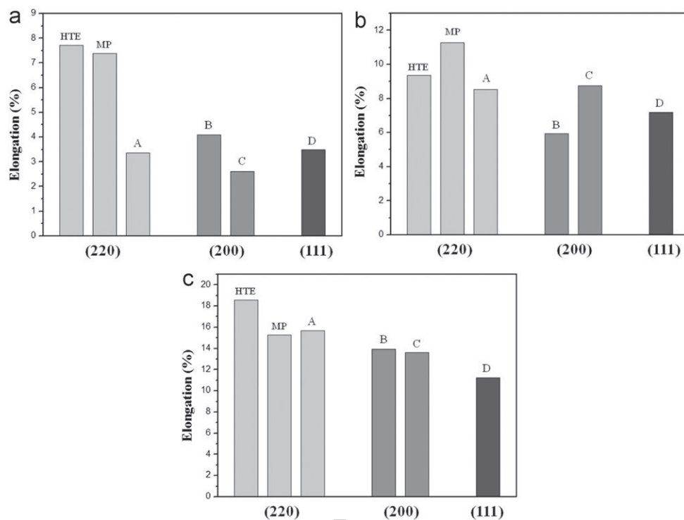
Fig. 13. Total elongation of the foils at different testing temperatures: (a) room temperature, (b) 150 °C and (c) 250 °C.
