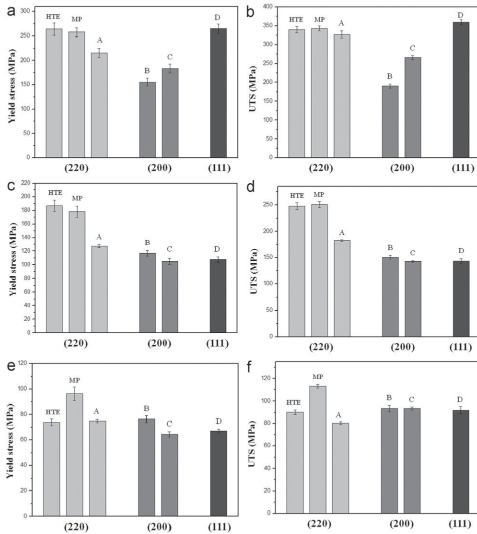
Fig. 12. Yield stress and ultimate tensile strength of the foils at different testing temperatures: (a and b) room temperature, (c and d) 150 °C and (e and f) 250 °C.
