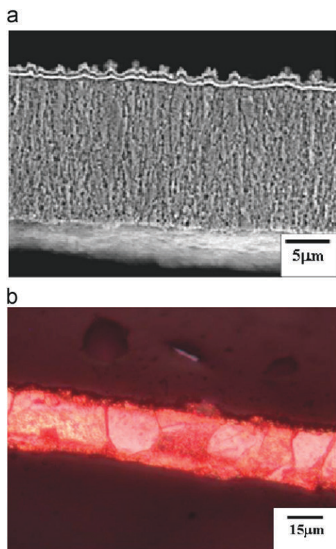
Fig. 6. VLP-D foils: (a) as-deposited samples with (111) preferred orientation, and (b) annealed samples.
