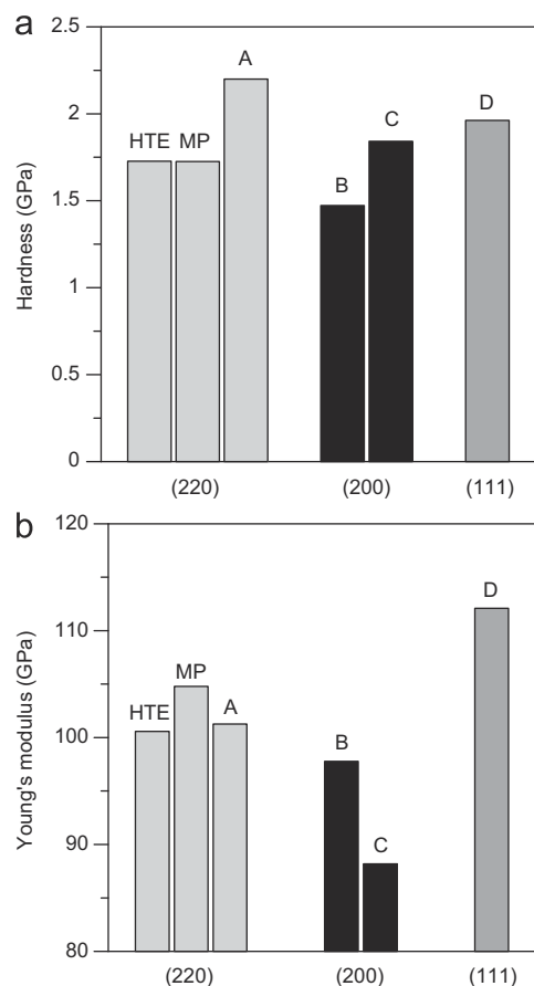
Fig. 10. Nanoindentation responses on the shiny side of the Cu foils: (a) hardness, and (b) Young's modulus.
