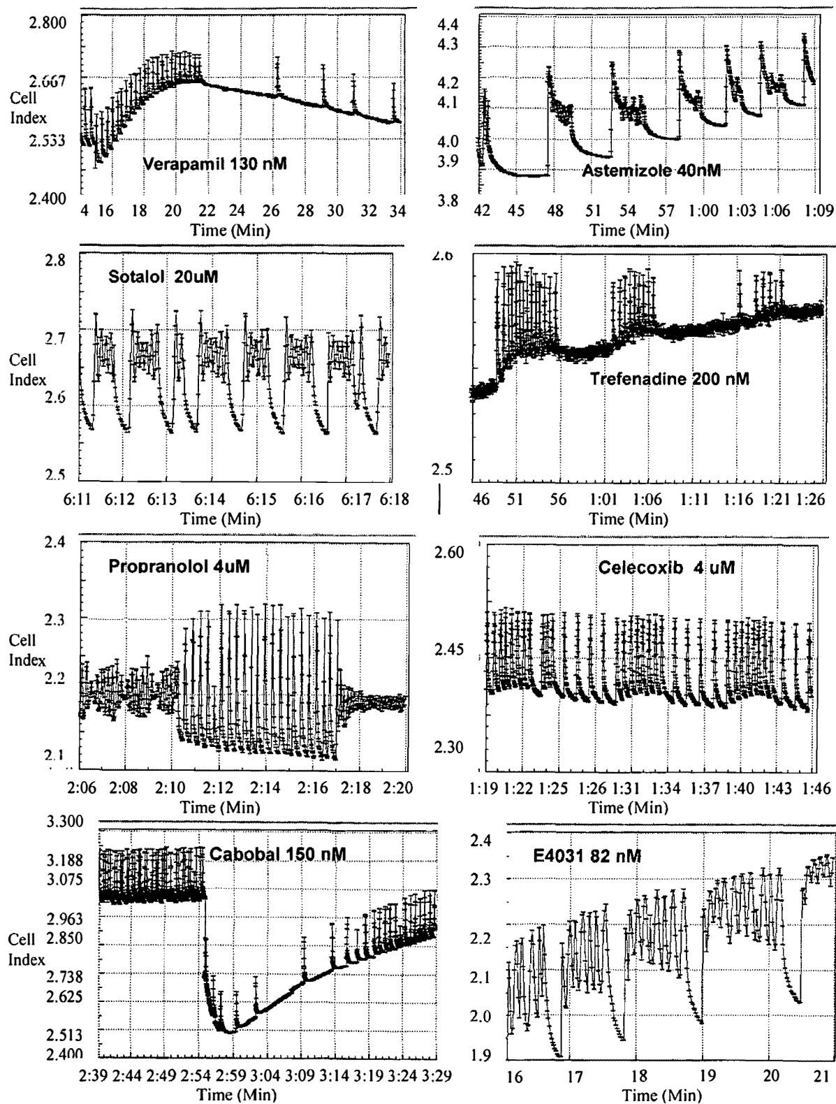
FIG. 12 Cardiotoxic Patterns
