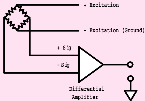
a. Strain Gage Sensor. CMV is equal to one-half the excitation.
