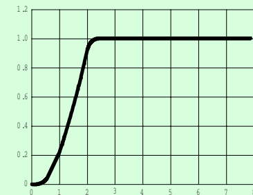
6-Pole Bessel
