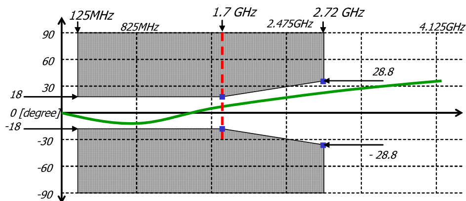
Figure G-2 Passive equalizer Cable Phase measurement method (explanation)
