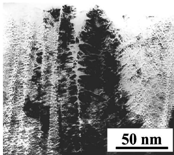
FIG. 8. Bright-field XTEM micrograph obtained from the top portion of a 3- \mu m -thick TiN film deposited on steel at 500^\circ C with a total pressure P_t = 38 mTorr. The ion-to-Ti flux ratio J_i/J_{Ti} incident at the film surface was 0.5 with an ion energy E_i = 100 eV.
