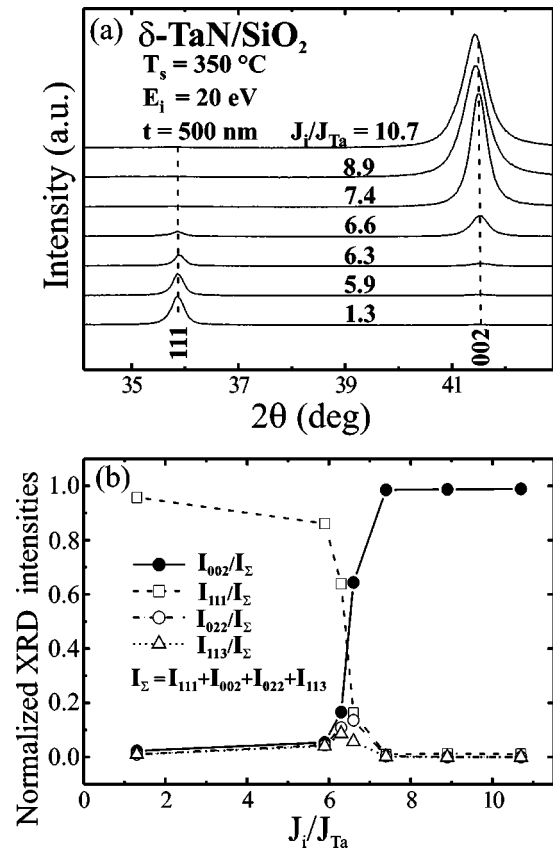
FIG. 12. (a) XRD \omega - 2\theta scans from 500-nm-thick \delta -Ta N layers grown by reactive magnetron sputter deposition on amorphous SiO 2 at 350 °C as a function of J_i/J_{Ta} with E_i = 20 eV. (b) Normalized intensities of the (111), (002), (022), and (113) XRD peaks in (a) as a function of J_i/J_{Ta} (see Ref. 90).
