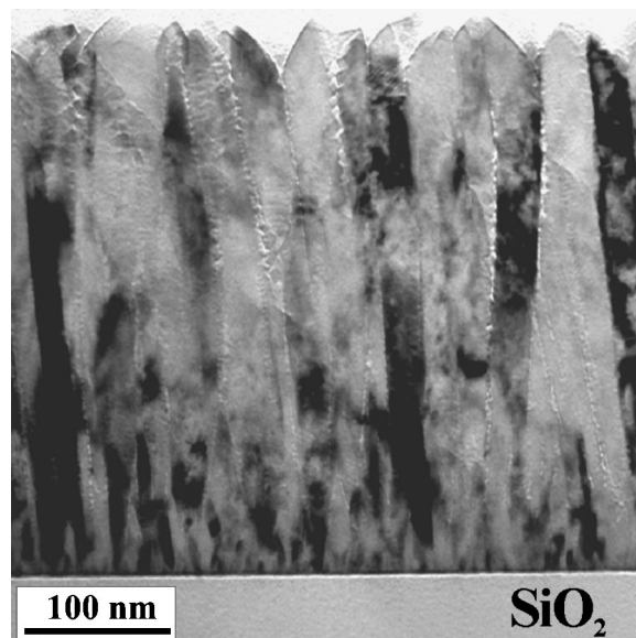
FIG. 9. Bright-field XTEM micrograph from a TiN film deposited on amorphous SiO_2 at 300^\circ C with a total pressure P_t = 5 mTorr. The ion-to-Ti flux ratio J_i/J_{Ti} incident at the growing film was \sim 1 with an ion energy E_i = 20 eV.
