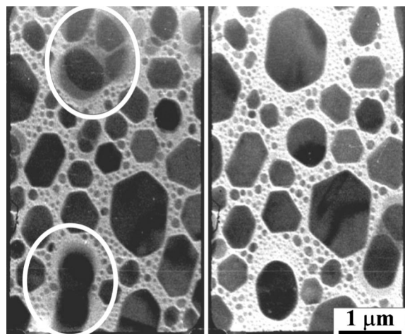
FIG. 2. In situ plan-view TEM micrographs obtained during the growth and coalescence of In islands deposited at 0.5 \text{ nm s}^{-1} on amorphous C substrates at T_s = 40^\circ\text{C} . The time lapse between obtaining the left and right images is 0.3 s. Note the denuded zones surrounding the coalesced islands (see Ref. 45).
