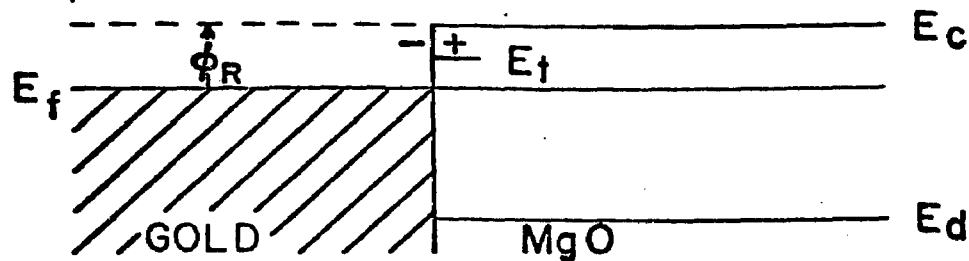
c. ENERGY BAND PICTURE FOR A GOLD-MgO INTERFACE WITH A HIGH DENSITY OF DONOR LIKE INTERFACE STATES
