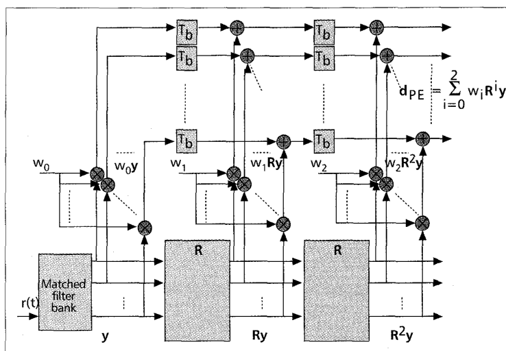
■ Figure 4. General DS-CDMA polynomial expansion detector with 2 stages.
