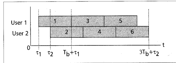
■ Figure 2. Sample timing diagram for an asynchronous channel. There are 2 users and 3 bits per user.
