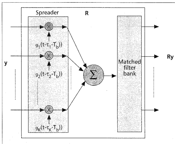
■ Figure 3. One stage of the polynomial expansion detector. The input is the matched filter bank output vector \mathbf{y} and the output is \mathbf{Ry} . A diagram of the matched filter bank is pictured in Fig. 1.
