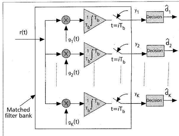
■ Figure 1. The conventional DS-CDMA detector: a bank of correlators (matched filters).
