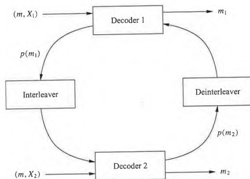
Figure 8.15: Turbo decoder.
