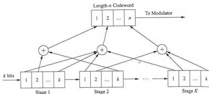
Figure 8.5: Convolutional encoder.
