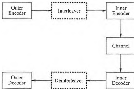
Figure 8.13: Concatenated coding.
