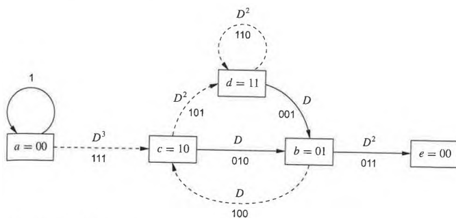
Figure 8.11: State diagram.
