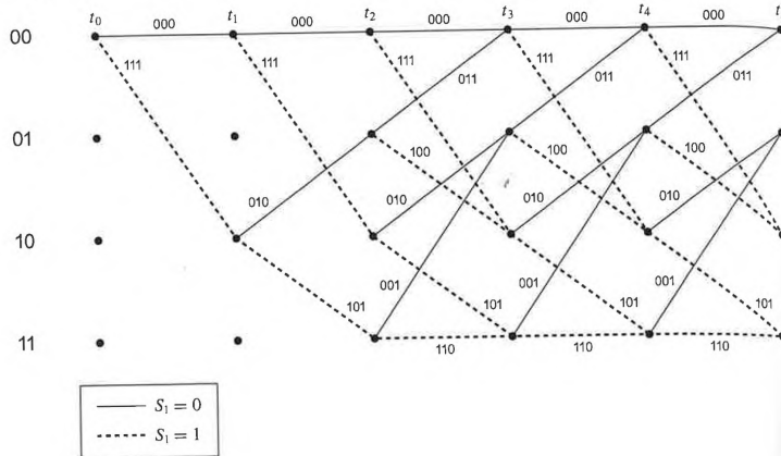
Figure 8.7: Trellis diagram.
