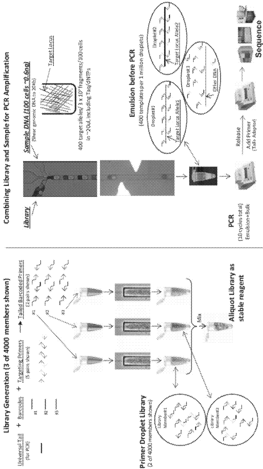
Figure 10 Single Molecule Barcoding for Haplotype Phasing: Overall Workflow
