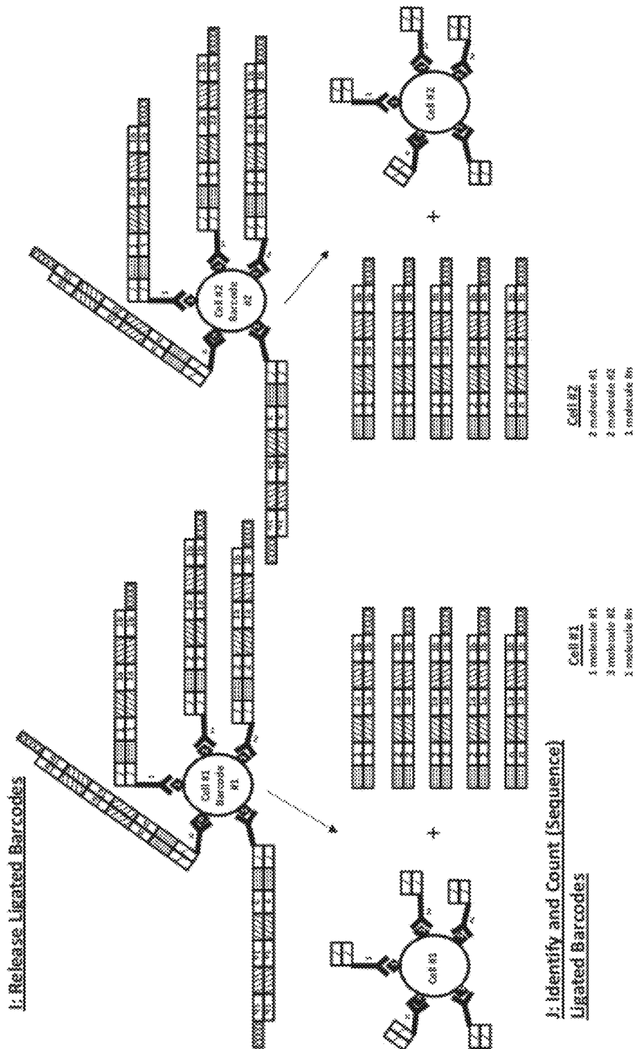
Figure 31 Universal Barcode Droplet Library: Single Cell Digital Biomarker Counting#4
