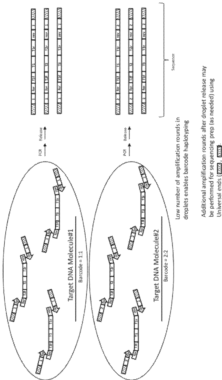
Figure 14 Universal PCR Barcode Library Single Molecule DNA Haplotyping 1.3
