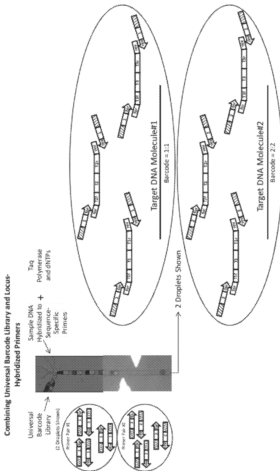
Figure 13 Universal PCR Barcode Library Single Molecule DNA Haplotyping 1.2
