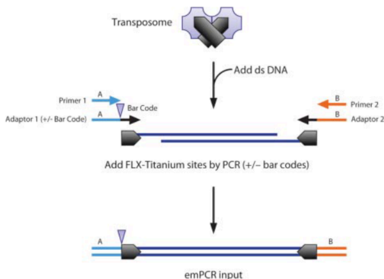
Fig. 19.2 Generation of Roche/454-compatible sequencing libraries. Target DNA is fragmented and tagged with the core Transposomes containing free transposon ends. Limited-cycle PCR with a four-primer reaction adds Roche/454-compatible adapters sequences. Optional barcoding (triangle) is added between the upstream emPCR adapter (blue) and the transposon end (gray).
