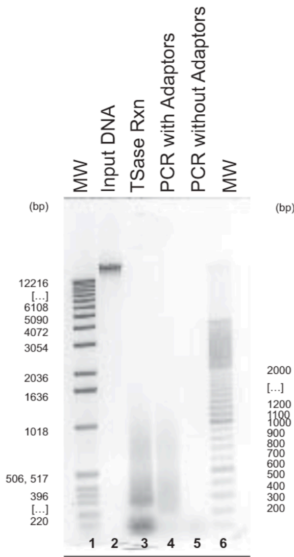
Fig. 19.5 Fragment size distribution of an Illumina GAIIx or HiSeq 2000-compatible sequencing library. HeLa DNA (lane 2) was tagmented with Illumina/Solexa-compatible Transposomes appended with sequencing tags (lane 3). Limited-cycle PCR added Illumina bPCR-compatible adaptors (lane 4). The recovered DNA was used directly in bPCR prior to sequencing on the Illumina GAII or HiSeq 2000 instrument. Control PCR without Adapter 1 and Adapter 2 (including Primer 1 and Primer 2) confirmed reaction specificity (lane 5).
