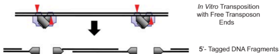
Fig. 19.1 Overview of Nextera fragmentation and tagging technology. Transposon integration and strand transfer occur via a staggered, double-stranded DNA break within the target DNA. When free transposon ends are used in the insertion reaction, the target DNA is cleaved and tagged at the 5' end with the transposon sequence. The resulting fragments have single-stranded gaps.
