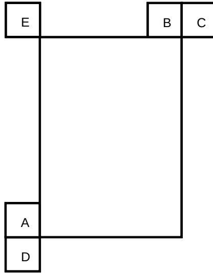
Figure 0-1 – Spatial neighbours that can be used as merging candidates (informative) illustrates the position of the spatial neighbours A, B, C, D and E relative to the current prediction unit.
